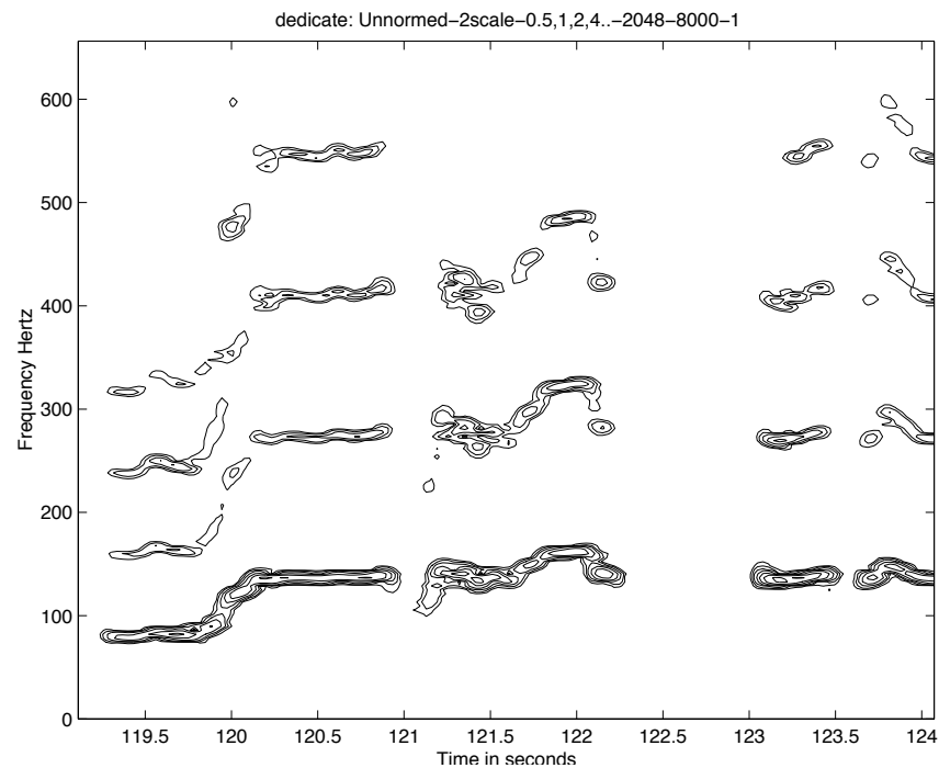
Figure 11: Frequency analysis of gospel quartet singing harmony.
