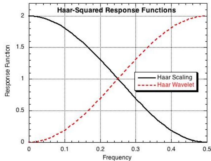
Figure 3. Haar scaling and wavelet responses, normalized as in (9.17). Usually we would divide by 2 to get a filter response of one at the maximum pass band.
