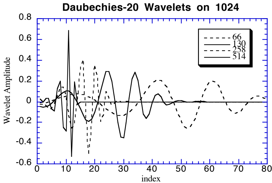
Figure 9. Daubechies wavelets at approximation condition 10.
