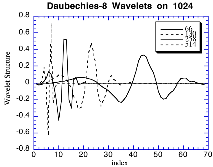
Figure 7. Daubechies wavelets at approximation condition 4.
