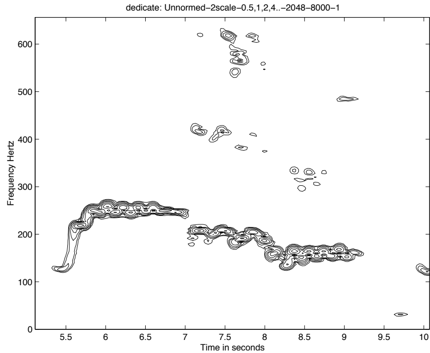
Figure10 : Frequency analysis of male vocalist. Contours are spaced in powers of two.
