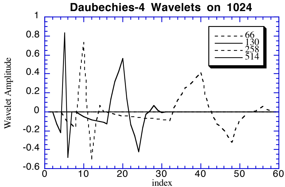
Figure 5. Examples of smallest scale Daubechies wavelets at approximation level 2, at detail levels 1,2,3, and 4.
