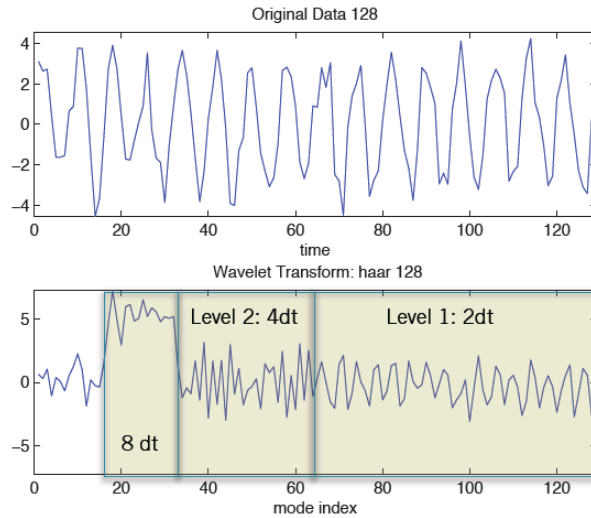
Figure 2. Time series with 8-day wave plus a bit of noise (top) and the Haar Wavelet transform of this time series (bottom). Because of the phasing of the 8-day wave, the third level of detail has an almost constant large projection on the data. The third level of detail is a Haar wavelet with a wave length of 8dt, and so projects strongly onto the sine wave with an 8-day period.
