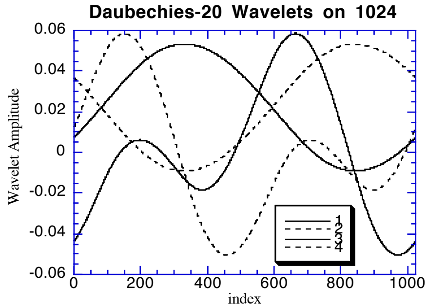
Figure 8. Daubechies wavelets at approximation condition 10.
