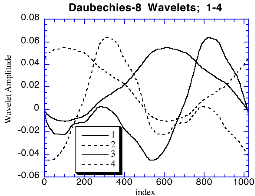
Figure 6. Daubechies wavelets at approximation condition 4.
