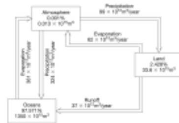
"Box Model" of the Water Cycle: Fig 4-22b
