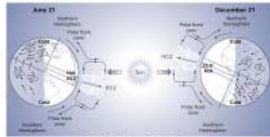
Hadley - seasonal movement: Fig 04_16
