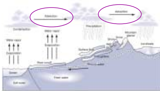
Water Cycle Picture: Fig 4-22a
