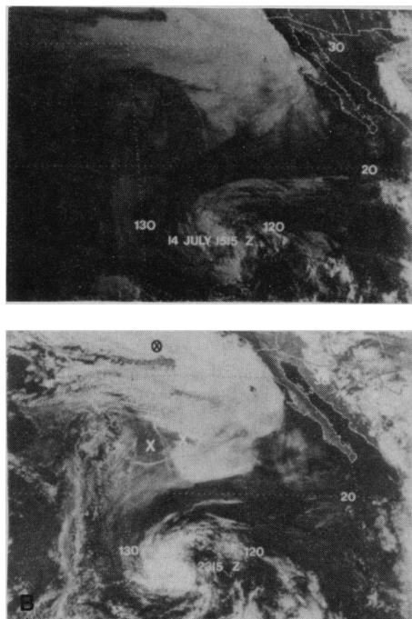
Fig. 2. Geostationary Operational Environmental Satellite (GOES) West visible images from 14 July 1987 at (A) 1515 UT and (B) 2315 UT showing ship trails in an “H” pattern. The X’s on the 2315 UT image indicate the location of the ship-trail intersections at 1515 UT. The ⊗ indicates the 1515 UT location of the eastern edge of an east-west band of clouds of low reflectivity that is located at about 32°N and 125°W.
