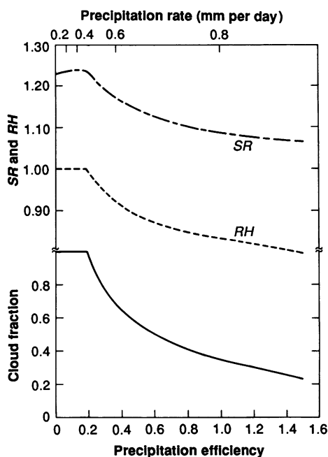
Fig. 4. The dependence of fractional cloudiness, RH , and SR for different specifications of a precipitation efficiency factor. The removal of water by precipitation processes in the parameterized convective elements by the model is assumed to be (dl/dz)_{\text{PRECIP}} = -a'l_c where z is height, l_c is the cloud liquid water, and a is the precipitation efficiency factor in units of per kilometer. A zero efficiency factor is no drizzle production and a value of a = 1 corresponds to a decrease in the cloud liquid water (for no condensation) by 1/e over a cloud depth of 1 km. Solutions are for the conditions described in Fig. 3 with a sea-surface temperature of 26^\circ\text{C} and D_0 of 5 \times 10^{-6} \text{ s}^{-1} .
