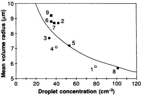
Fig. 1. Droplet concentration as a function of the mean volume droplet radius r_v for droplets in the range of r = 1 to 16\ \mu\text{m} . For a given liquid-water content L and number density N , L = (4/3)\pi r_v^3 \rho N , where \rho is the density of water (4). Measurements were obtained during aircraft ascents and descents made with the National Center for Atmospheric Research (NCAR) Electra during FIRE (20) in horizontally homogeneous clouds ranging in depth from 150 to 500 m in June and July of 1987 at locations about 400 to 500 km southwest of Los Angeles. The values are averages over a 20-m layer centered 100 m above cloud base and were made with a Particle Measurements Systems (PMS) forward scattering spectrometer probe where L = (4/3)\pi \rho \sum r_i^3 N_i , and the sum is over different droplet sizes sampled. The solid line shows the relation between N and r_v for a constant L of 0.08\ \text{g g}^{-3} . Numbers refer to cases in Table 1. The shaded symbols correspond to the cases where drizzle (●) or significant drizzle (■) as defined in Table 1 was observed.
