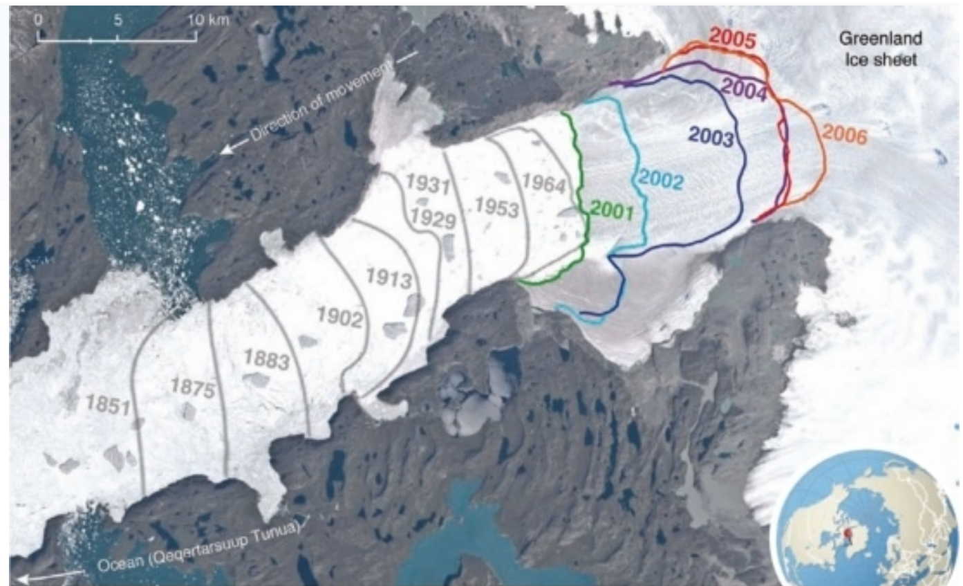
Figure 6A.6: Landsat satellite image of Jakobshavn Isbrae and its fjord, showing locations of the calving ice front in years from 1851 to 2006. The glacier extends through the Illulisat Icefjord, surrounded by mountains. Icebergs calve off from the main glacier, pile up and block the fjord before being released into Qeqertarsuup Tunua (Disko) Bay and Davis Strait. The whiter areas in the fjord are piled-up icebergs and the "real" glacier ends where the greyish striped section ends – showing that this image is from 2001. The graph shows glacier-velocity profiles for 1985 to 2006. During this period Jakobshavn Isbrae, already the world's fastest glacier, doubled its speed to almost 14 km per year 28,29 after rapid thinning and break up of its floating ice tongue 31 .
