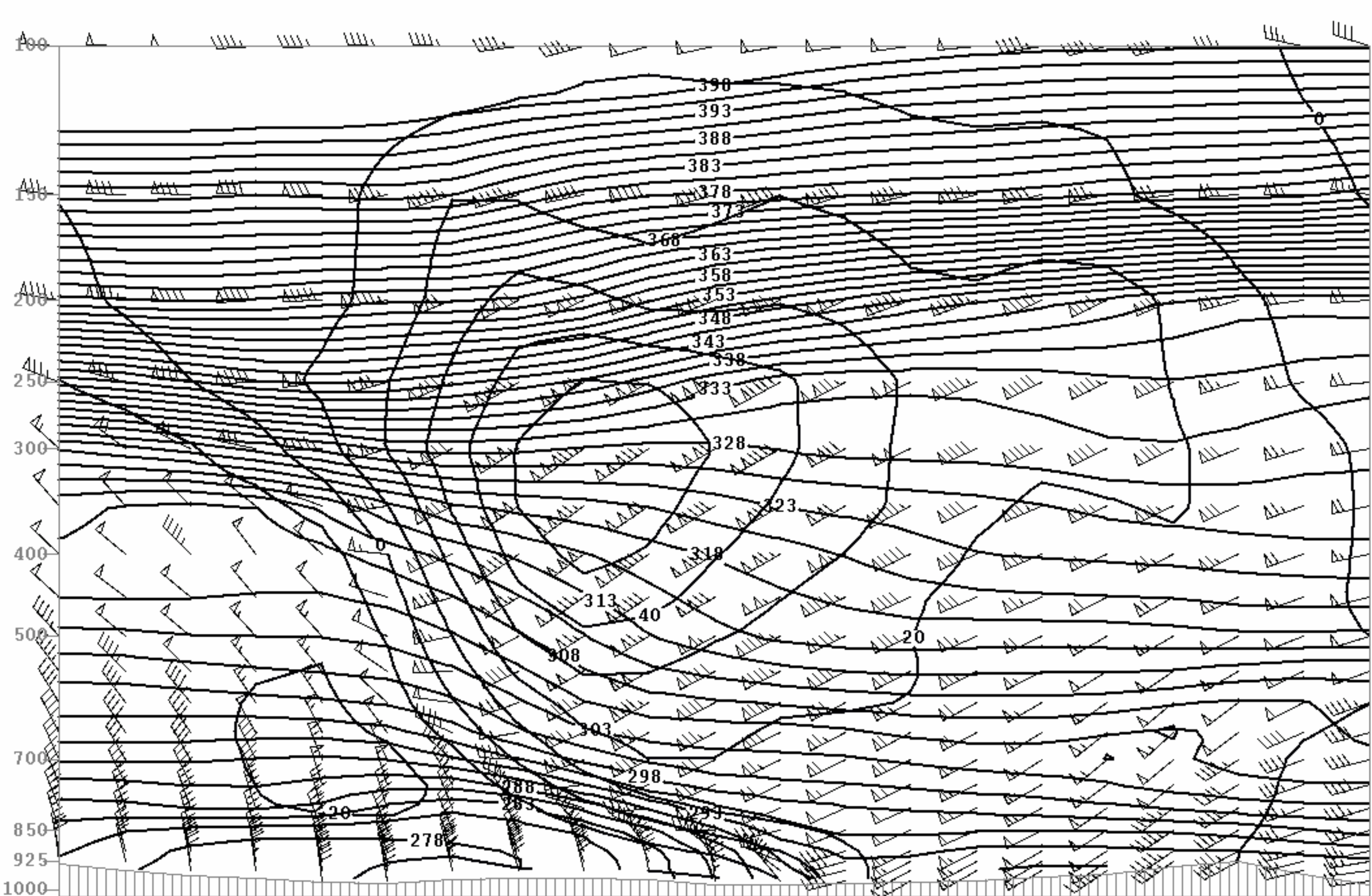
TUE Feb 04 2003 0000V000 AVN Scalar Normal Wind TUE Feb 04 2003 0000V000 AVN Geostrophic Wind TUE Feb 04 2003 0000V000 AVN Potential Temperature
