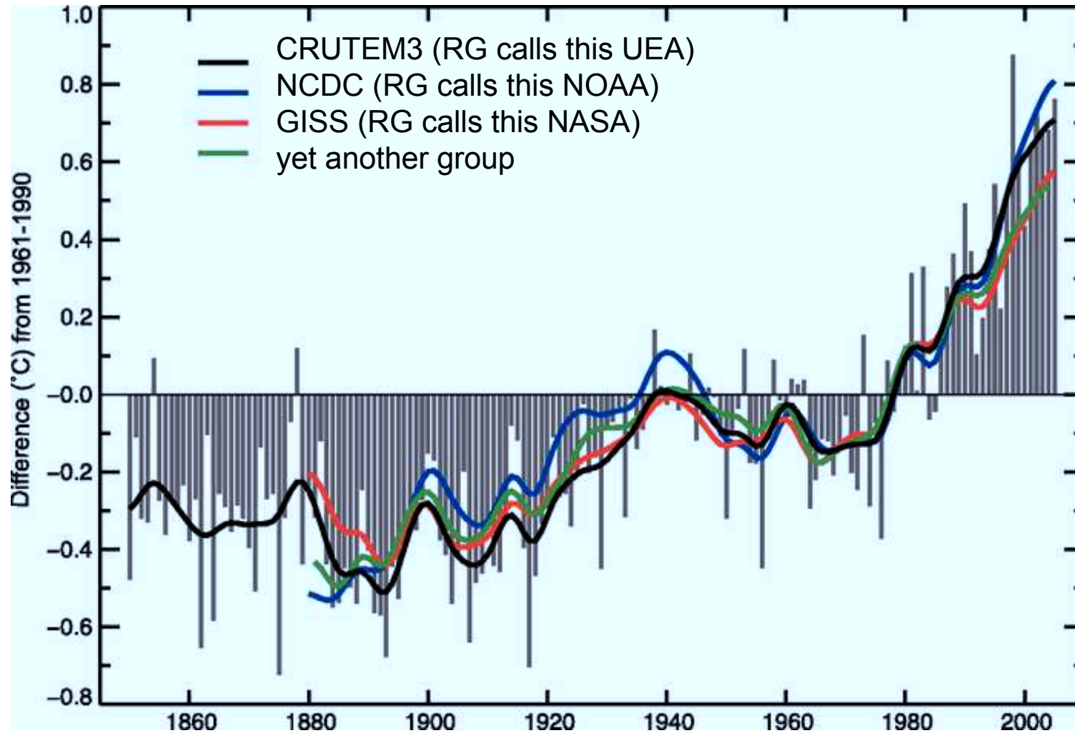
Figure 3.1 from 2007 IPCC
