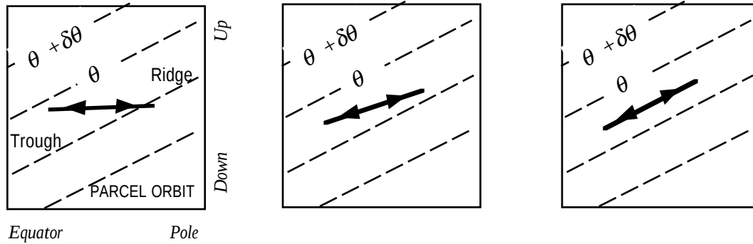
Fig. 5.4 Idealized orbits or trajectories of air parcels in waves in which the streamline and temperatures are in quadrature. Left: horizontal motion. Right: trajectories parallel to the isentropes. Middle: an intermediate slope.
