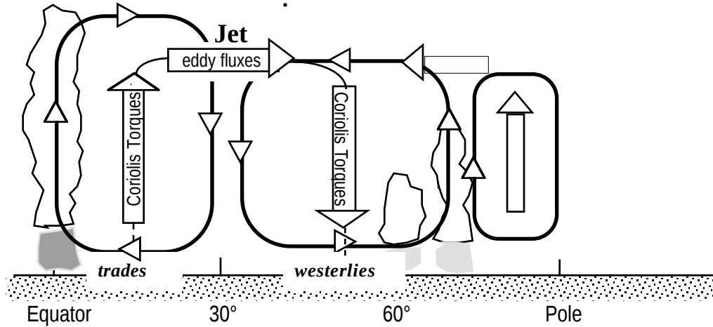
Fig. 2.16 Schematic of the transport of atmospheric angular momentum in the earth's atmosphere.
