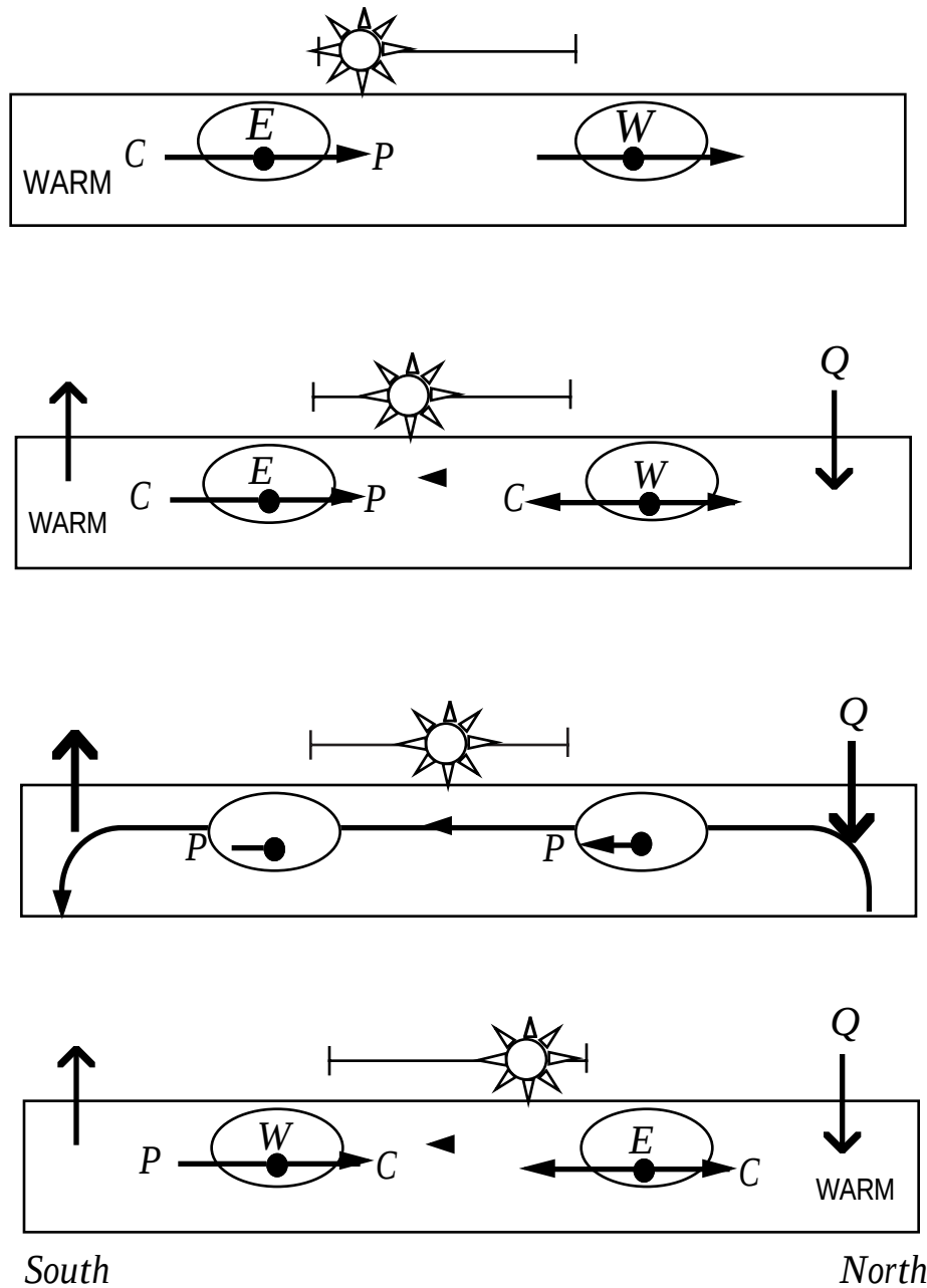
Fig. 4.2 Schematic of the seasonal evolution of the zonally averaged circulation in the mesosphere showing the jets (W, E), the pressure gradient (P) and Coriolis (C) forces, the diabatic heating (Q), the latitude at which the sun is overhead, and the mean meridional circulations, indicated by the cell. Intensity is indicated by line width and the thickness of the labels. The sections extend from pole to pole and from 30 to 80 km.
