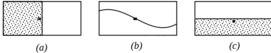
Fig. 1.1 (a) Heavier (shaded) and lighter fluids separated by a movable partition. The dot represents the center of gravity of the two-fluid system. (b) Fluids in motion following the removal of the partition. (c) Equilibrium configuration of the fluids after the motion has been dissipated by friction.
