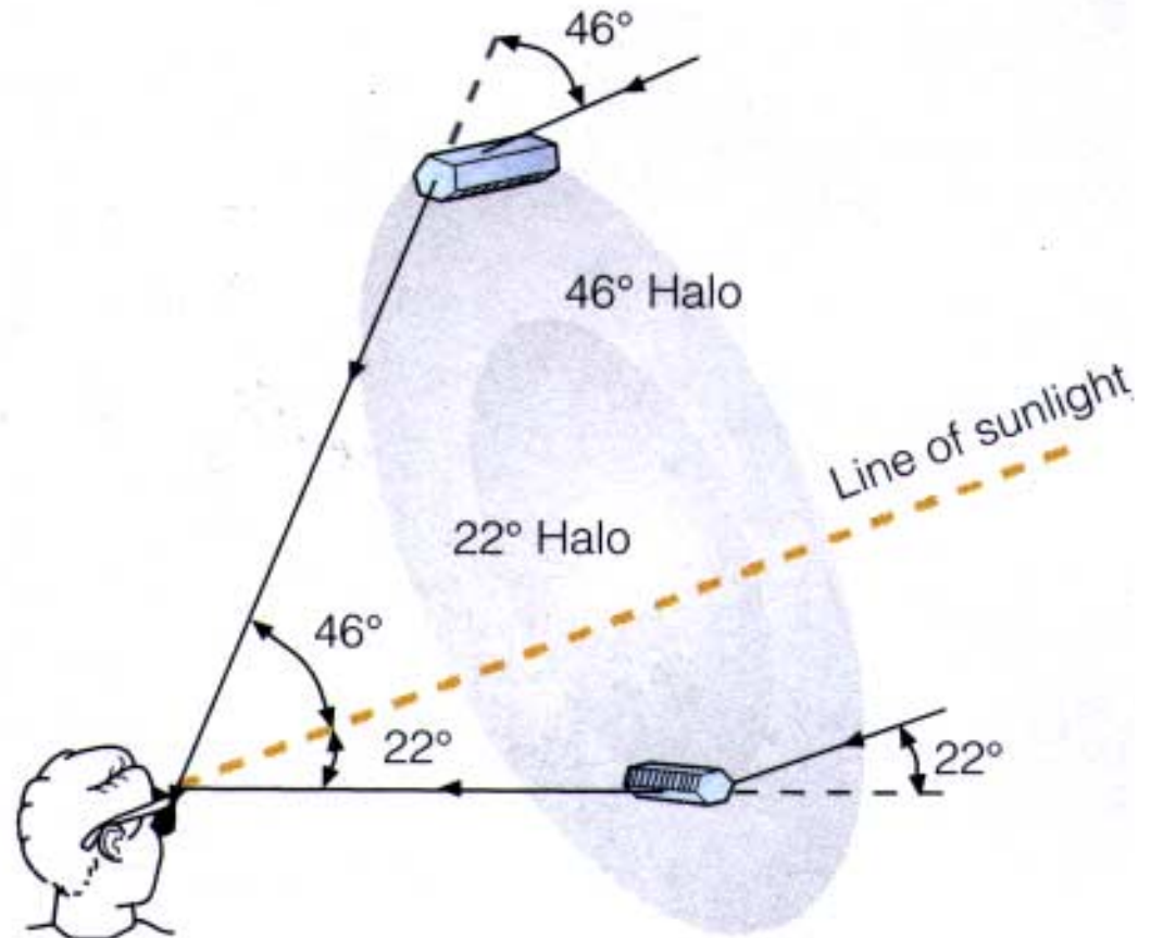
Figure 15.16 EOM 15.18 The formation of a 22° and a 46° halo.
