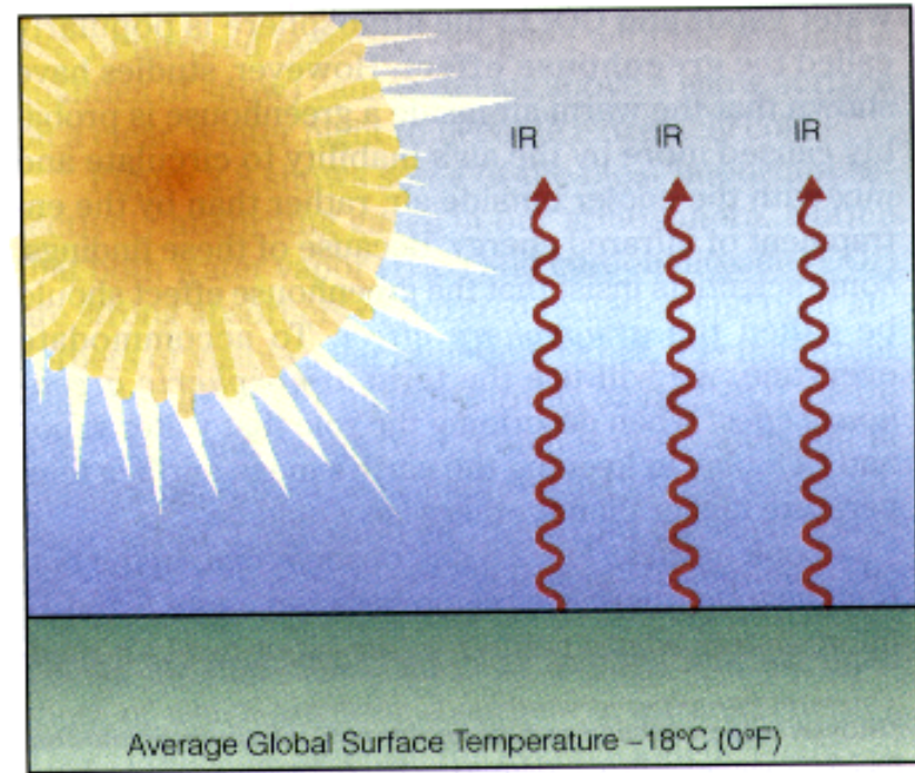
(b) Earth's atmosphere without H 2 O and CO 2 EOM 2.10
