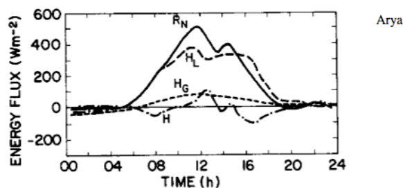
Fig. 2.4 Observed diurnal energy budget of a barley field at Rothamsted, England, on July 23, 1963. [From Oke (1987); after Long et al. (1964).]
