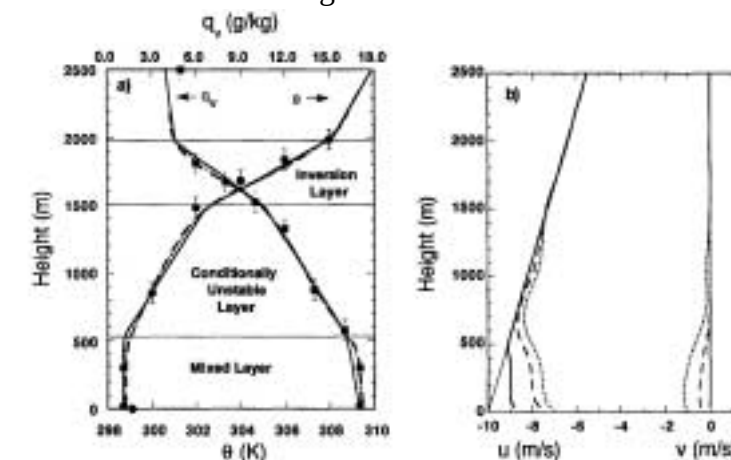
FIG. 1. Horizontally averaged vertical profiles of \theta and q , (a) and the u and v components of the velocity (b) at time t = 0 h (solid line), t = 3 h (dotted line), and t = 7 h (dashed line). The circles and squares are the observed values. The thin line in (b) is the geostrophic wind profile.
