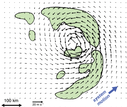
(a) 500 mb
