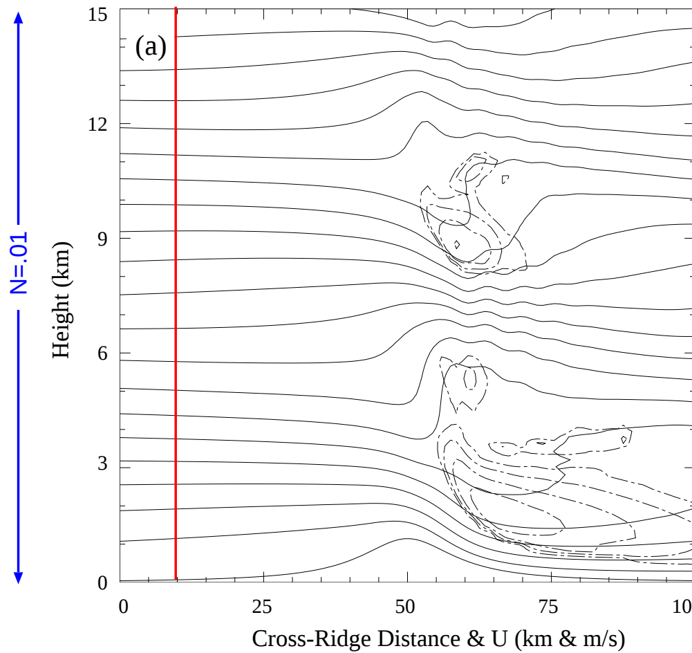
Uniform Vertical Structure
