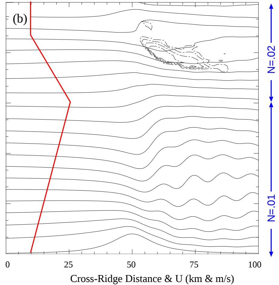
Vertical Shear and a Stratosphere
