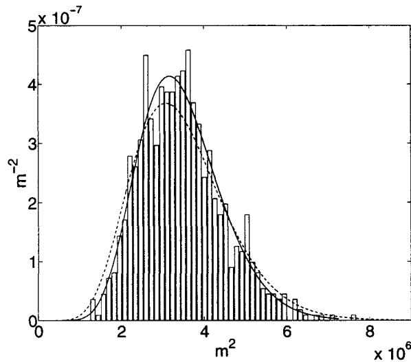
FIG. 4. \chi^2 distributions with N_{mm}^* = 23.8 (solid) and N_{ef}^* = 18.5 (dashed) degrees of freedom superposed on the observed frequency distribution of spatially averaged 500-mb height variance.
