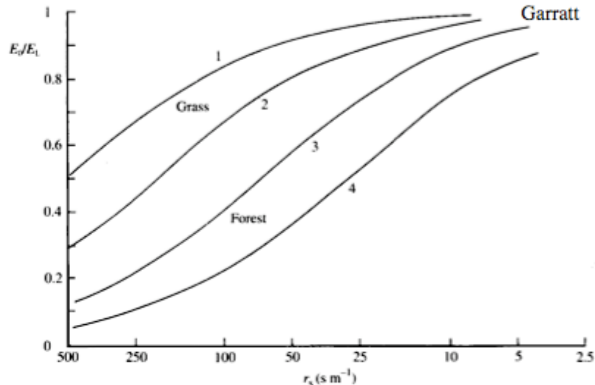
Fig. 5.8 Variations of E_0/E_L (Eq. 5.37) with surface resistance. Values of r_{av} have been calculated for neutral conditions, with z_q = z_0/7.4 . For short grass ( z_0 = 0.0025 m): curve 1, T = 303 K; curve 2, T = 278 K. For forest ( z_0 = 0.75 m): curve 3, T = 303 K; curve 4, T = 278 K.
