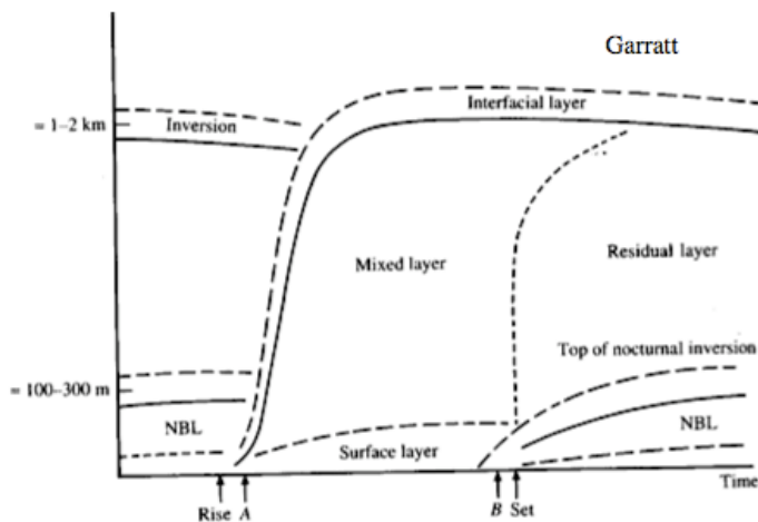
Fig. 6.1 Schematic representation of ABL evolution throughout the diurnal period over land under clear skies.
