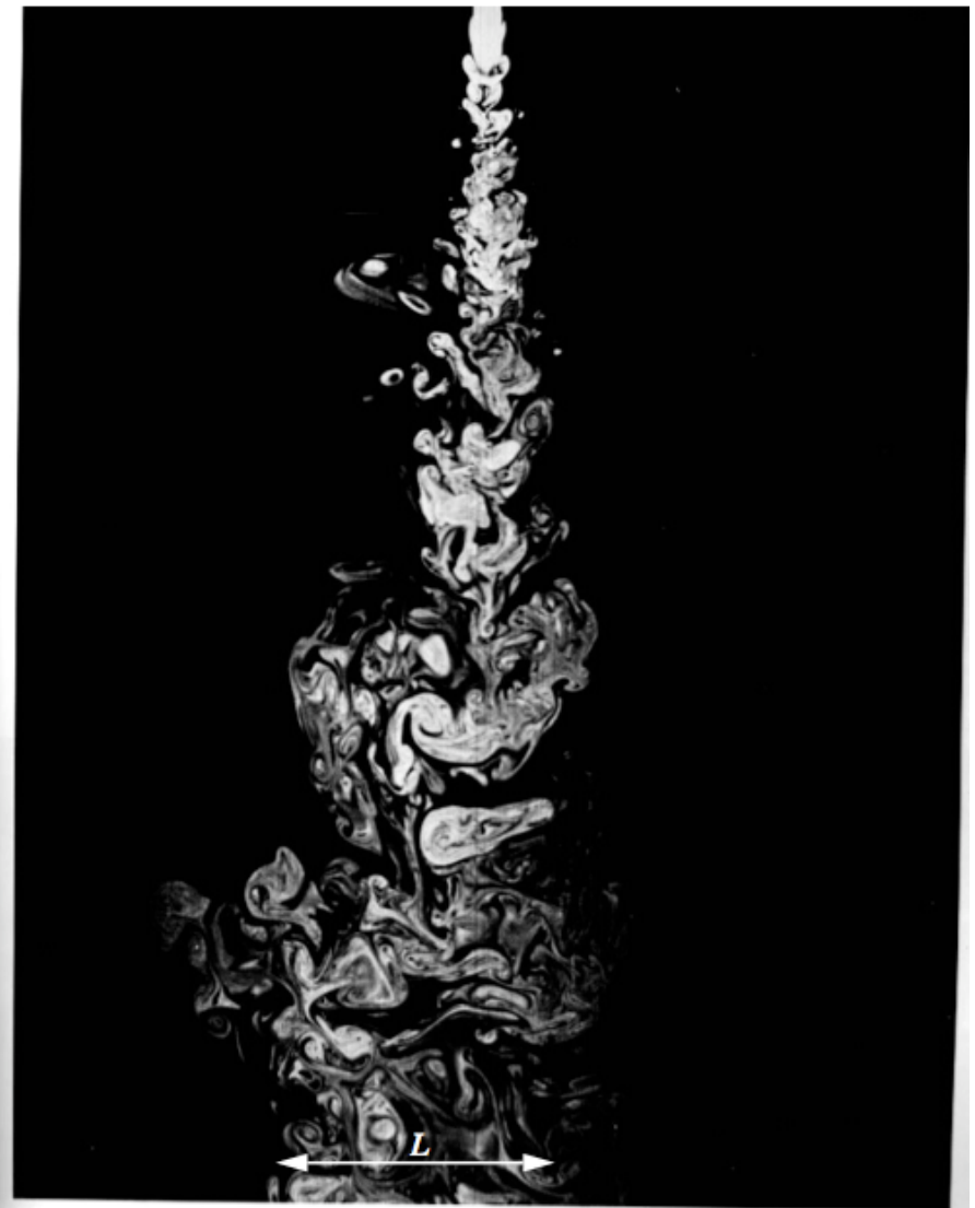
166. Turbulent water jet. Laser-induced fluorescence shows the concentration of jet fluid in the plane of symmetry of an axisymmetric jet of water directed downward into water. The Reynolds number is approximately 2300.
