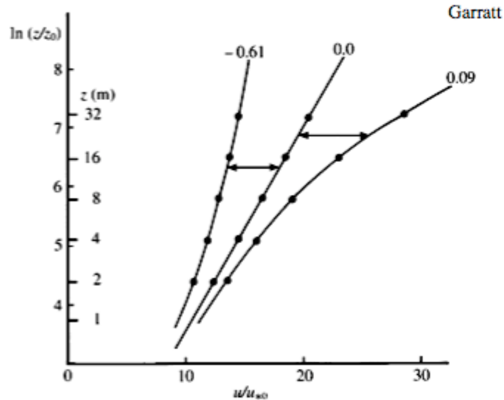
Fig.3.5 Three wind profiles from the Kansas field data (Izumi, 1971) plotted in normalized form at three values of the gradient Ri ( z = 5.66 m). Both normalized and absolute heights are shown, whilst the magnitude of the horizontal arrows indicates the effect of buoyancy on the wind relative to the neutral profile (see Eq. 3.34).
