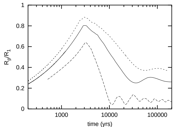
FIG. 3.—Evolution of the pulsar nebula through the return of the reverse SNR shock for the three different models listed in Table 1: model A (solid), model B (long-dashed line), and model C (short-dashed line). The radius of the pulsar nebula is scaled to the (increasing) radius of the SNR as in the previous figure.
