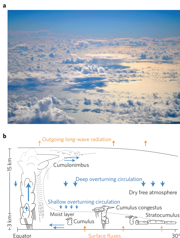
Figure 1 | What role does convection play in cloud feedbacks? a , Shallow convective clouds, with tops around 2.5 km, photographed over the tropical North Atlantic. Climate models are very sensitive to how such clouds are coupled to the larger-scale circulation, the vertical distribution of water vapour, surface turbulent fluxes and atmospheric radiation. b , This coupling links regions of shallow convective clouds to remote areas of deep convection (hints of which can also be seen in the background of a ). Image in a courtesy of Bjorn Stevens.
