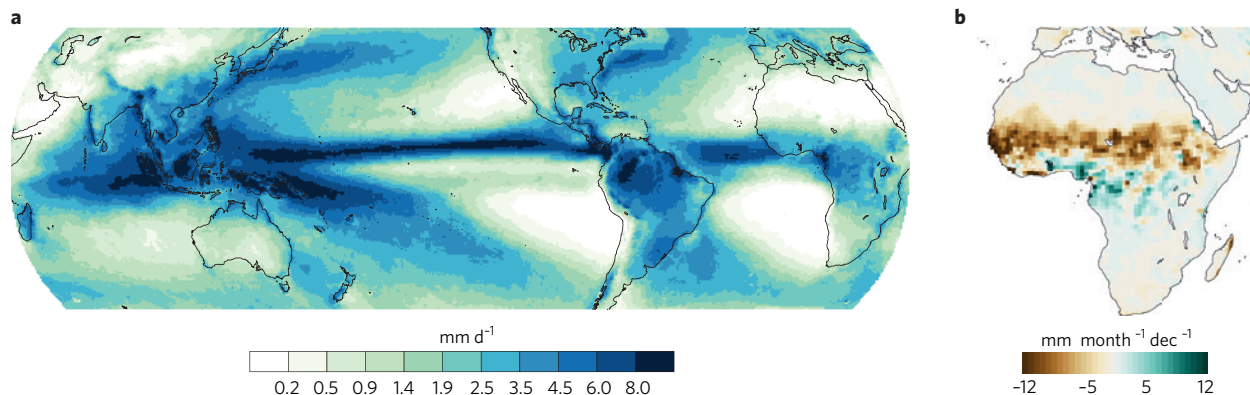
Figure 3 | What controls the position, strength and variability of tropical rain belts? a , Observations over the period 1998–2005 (derived from the satellite Tropical Rainfall Measuring Mission) feature a contrasted distribution of precipitation at the regional scale, with large amounts of rainfall occurring in narrow bands of the tropics. b , The position of tropical rain bands has a pronounced influence on precipitation over land, with droughts over periods of decades attributable to shifts in the ITCZ, as seen for instance in the Sahel during the twentieth century 34 . Colour scale shows the observed decadal trend in Sahel wet season (July–September) precipitation rate between 1950 and 2000. Panel a © Tropical Rainforest Mission/Nasa. Panel b reproduced with permission from ref. 34, PNAS.
