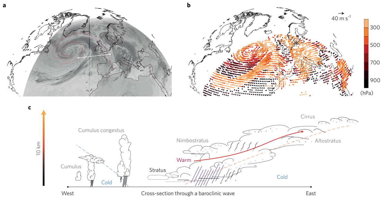
Figure 2 | What controls the position, strength and variability of storm tracks? a , Infrared radiances visualize patterns of clouds in a developing storm whose wavelike structure is outlined by red contour delineating air-mass boundaries in upper troposphere. b , Cloud motion vectors, coloured by cloud-top pressure, derived from radiances. c , Conceptual cartoon illustrating major cloud types along a cross-section through the storm system. In a and b the data are from 5 January 2014 and limited by the field of view of the Meteosat satellite. Panel a,b © 2015, EUMETSAT.
