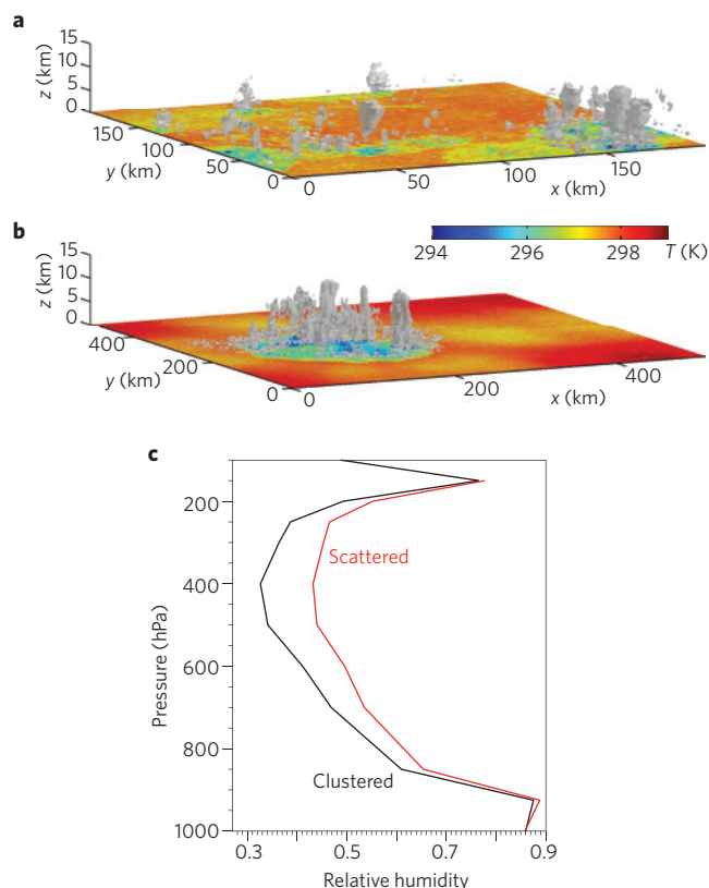
Figure 4 | What role does convective aggregation play in climate? In models, convective organization can exhibit a random distribution (a) or evolve spontaneously towards an aggregated state (b) 42 , increasingly so with increasing temperature 40 . c. In observations (relative humidity profiles from AIRS satellite measurements), the middle troposphere is drier in an atmosphere in which the same amount of precipitation is concentrated in a smaller number of convective clusters 39 . Figure reproduced with permission from a,b, ref. 42, AMS; c, ref. 39, AMS.
