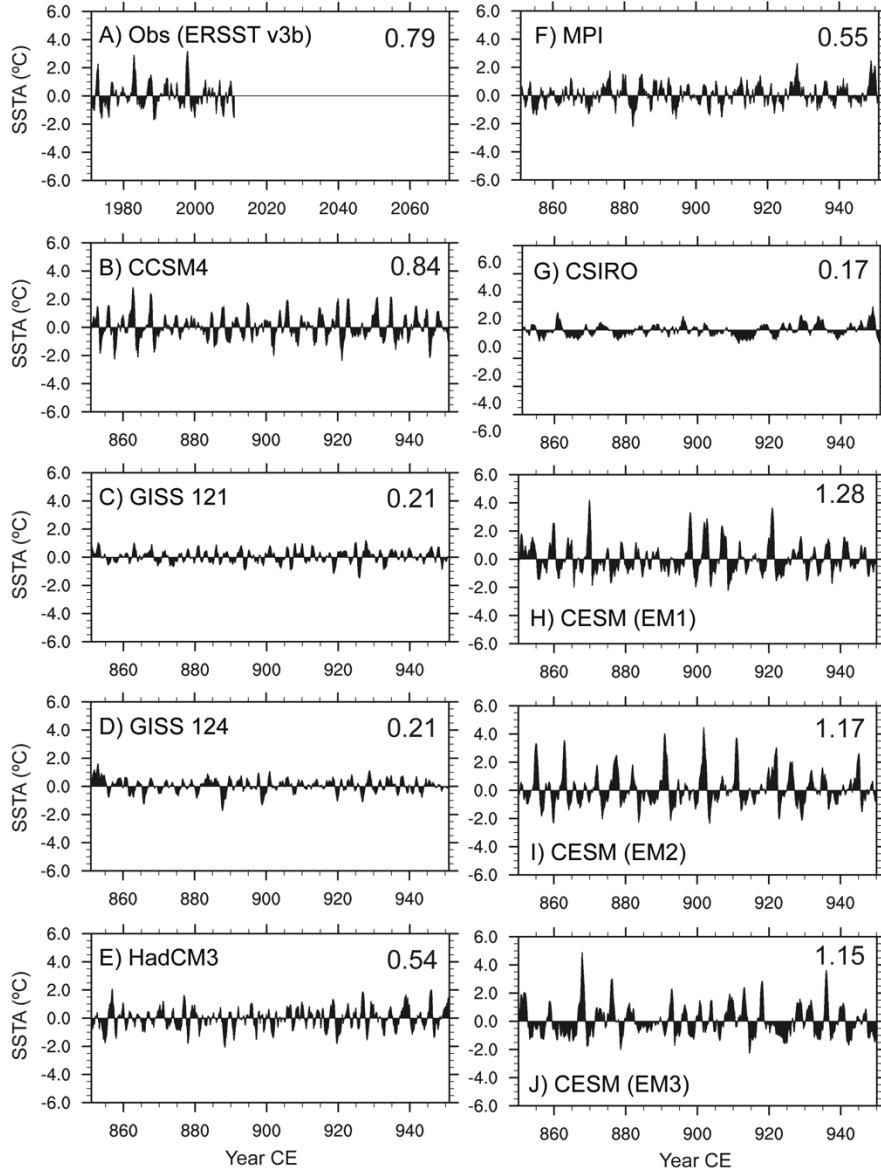
Figure S11. Time series of 3-month running mean Niño 3 SSTAs in (A) observations (ERSST v3b; 1971–2010), (B–G) the first 100 years of the CMIP5/PMIP3 last millennium simulations, and (H–J) the first 100 years of ensemble members 1–3 of the CESM LME. The variance of each time series (1971–2010 for the observations and all 1,000 years of the model simulations) is indicated in the right corner of each panel.
