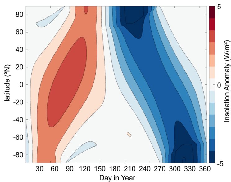
Figure S2. Insolation difference between the LIA (1450-1850 CE) and MCA (950-1200 CE) in \text{W/m}^2 as a function of latitude and Julian day. Data were derived from the Berger et al. (1978) equations.
