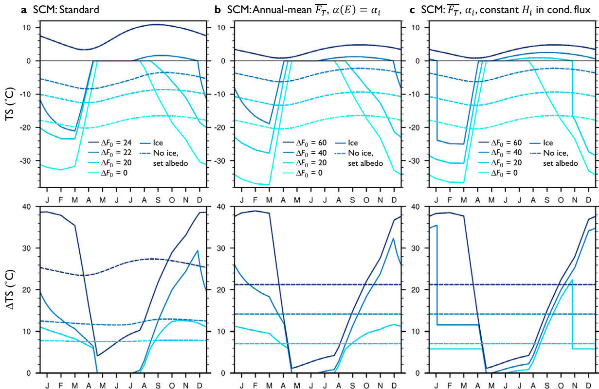
FIG. 4. (top) As in Figs. 2b–d for select surface forcing experiments, solid lines show surface temperature (TS; °C) in (a) the standard SCM, (b) the SCM with annual-mean \overline{F_T(t)} and constant \alpha(E) = \alpha_i , and (c) the SCM with annual-mean \overline{F_T(t)} , constant \alpha(E) = \alpha_i , and constant ice thickness H_i when calculating the conductive heat flux through frozen ice, which is set to the annual-mean H_i from the \Delta F_0 = 0 experiment with annual-mean \overline{F_T(t)} and constant \alpha(E) = \alpha_i . Dashed lines show TS for identical experiments, but with a mixed layer SCM and prescribed surface albedo from the experiments with ice. (bottom) TS anomalies compared to the \Delta F_0 = 0 experiment. Note that TS is identical in the Ice and No ice, set albedo experiments for the highest forcing experiment, which is annually ice-free.
