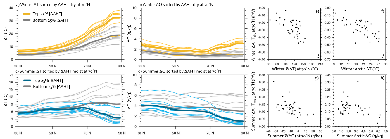
Figure 3. Anomalies in (a, c) near-surface temperature ( \Delta T ; ^{\circ}\text{C} ) and (b, d) specific humidity ( \Delta Q ; \text{g/kg} ) in \text{CO}_2 quadrupling simulations in Coupled Model Intercomparison Project phase 6 (CMIP6) for the top and bottom 25% of models sorted by their change in (a, b) winter dry and (c, d) summer moist atmospheric heat transport (AHT) for individual models (thin lines) and their ensemble means (thick lines). Change in winter dry AHT (PW) versus (e) the gradient in \Delta T at 70^{\circ}\text{N} ( ^{\circ}\text{C}/\sin \theta ; r^2 = 0.59 ) and (f) Arctic \Delta T ( ^{\circ}\text{C} ; r^2 = 0.54 ), and change in summer moist AHT (PW) versus (g) the gradient in \Delta Q at 70^{\circ}\text{N} ( \text{g/kg}/\sin \theta ; r^2 = 0.35 ) and (h) Arctic \Delta Q ( \text{g/kg} ; r^2 = 0.09 ) for \text{CO}_2 quadrupling simulations in 41 CMIP6 models.
