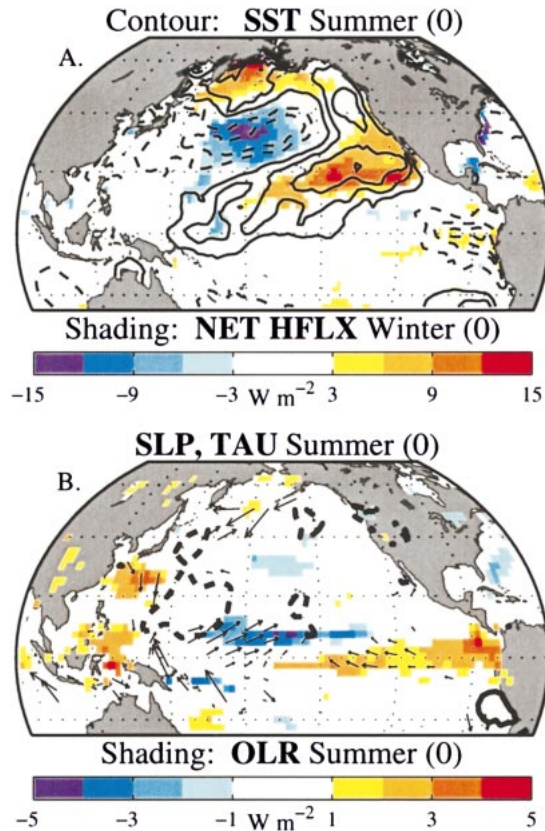
FIG. 4. (a) Regression maps of summer (0) SST (with summer CTI linearly removed) [contours; contour interval 0.075^{\circ}\text{C} (std dev) ^{-1} ] shown together with the winter (0) net surface heat flux (shading). Both fields are regressed onto the winter (0) WIN_NPO index. The net heat flux is shown only where the correlation is significant at the 95% confidence level. (b) Summer (0) OLR (shading), and wind stress (vectors) regressed onto the winter (0) WIN_NPO index. Also contoured is the \pm 0.4 correlation between summer (0) SLP and WIN_NPO. OLR and wind stress are shown only where OLR and surface wind speed are significantly correlated with WIN_NPO at the 90% and 80% confidence levels, respectively. An SLP correlation of 0.4 is significant at the 90% level over most of the domain. All maps in (b) are generated using the 1979–2001 record.
