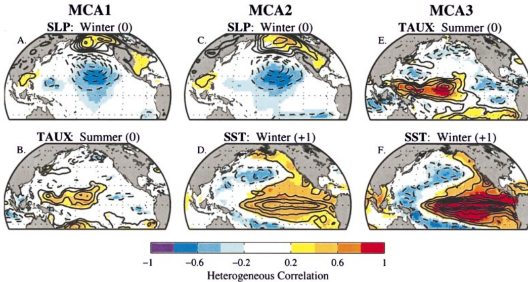
FIG. 3. Leading heterogeneous patterns for the three separate MCA sets described in Fig. 2: (a), (b) SLP and zonal wind stress, respectively, from MCA1; (c), (d) SLP and SST from MCA2; (e), (f) zonal wind stress and SST from MCA3. Units are 0.20 \text{ hPa (std dev)}^{-1} for SLP; 0.02 \text{ dyn cm}^{-2} (\text{std dev})^{-1} for zonal wind stress; 0.15^\circ\text{C (std dev)}^{-1} for SST. Positive contours are solid, negative contours are dashed, and the zero line has been omitted. The correlation coefficient is shaded and is displayed only where it exceeds the 95% confidence level, based on a two-tailed Student's t test.
