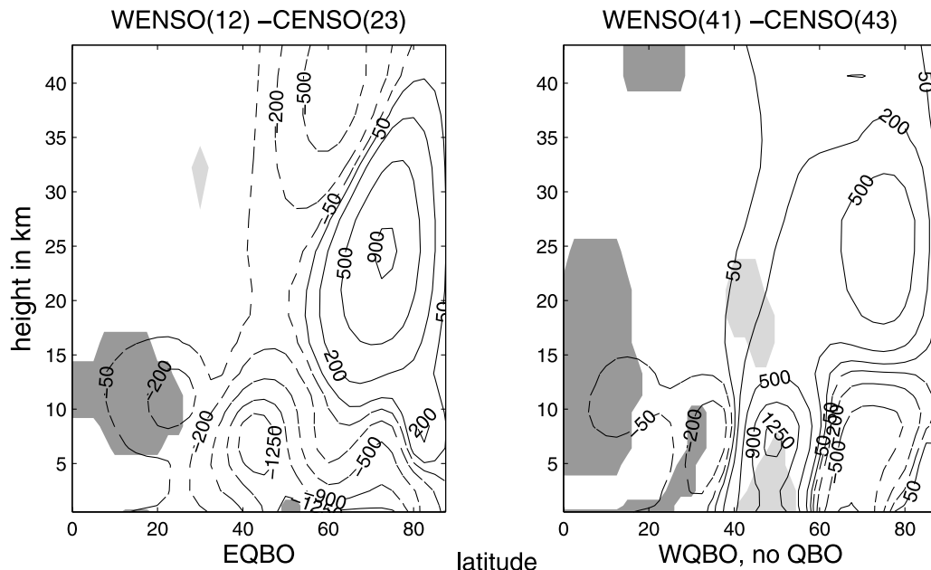
Figure 9. The difference in wave 1 height variance between WENSO and CENSO in NDJF over the NH. (left) EQBO and (right) WQBO or no QBO (limit combination: |\text{ENSO}| > 0.6 , \text{QBO} < -0.6 in Figure 9 (left) and \text{QBO} > -0.4 in Figure 9 (right)). Plotting conventions as in Figure 5.
