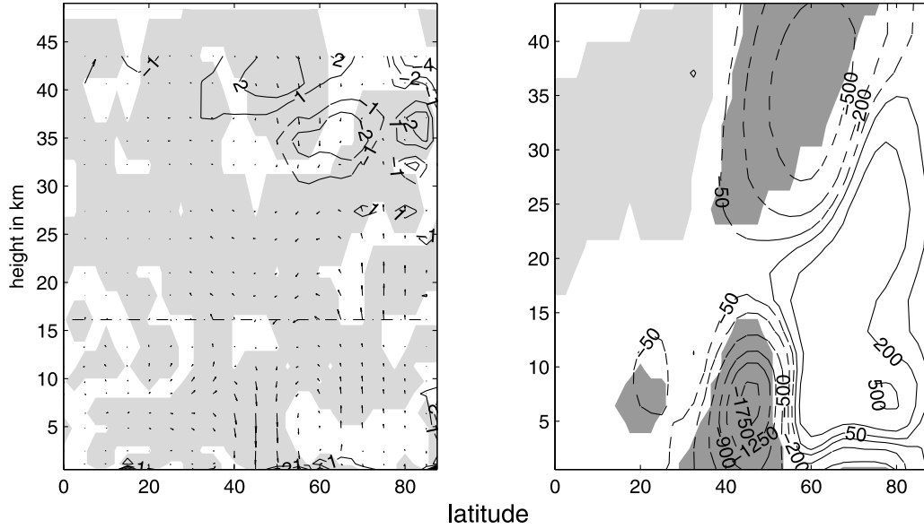
Figure 10. (left) The difference in wave 1 EP flux between EQBO and WQBO under WENSO. (right) wave 1 variance of the height. As in GH07, ONDJ is examined. A month with QBO or ENSO index greater than 0.6 standard deviations is composited as ENSO or QBO. Plotting conventions as in Figures 2 and 5.
