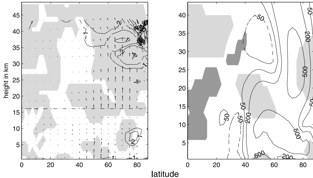
Figure 11. The difference between EQBO and WQBO under CENSO. (left) wave 1 EP flux and (right) wave 1 variance of the height. As in GH07, the months of ONDJ are examined. A month with QBO or ENSO index greater than 0.6 standard deviations is composited as ENSO or QBO. Plotting conventions as in Figures 2 and 5.
