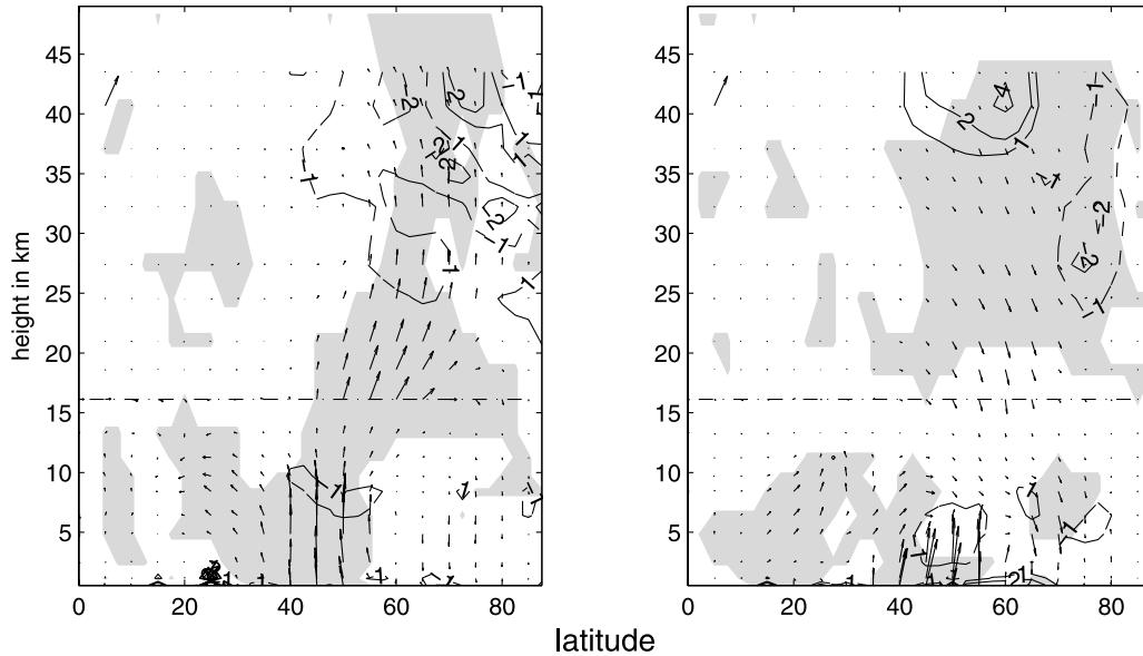
Figure 3. Difference in EP flux between WPNA and CPNA. (left) Wave 1 and (right) wave 2. Only neutral ENSO months but all QBO phases are included. Plotting conventions as in Figure 2.
