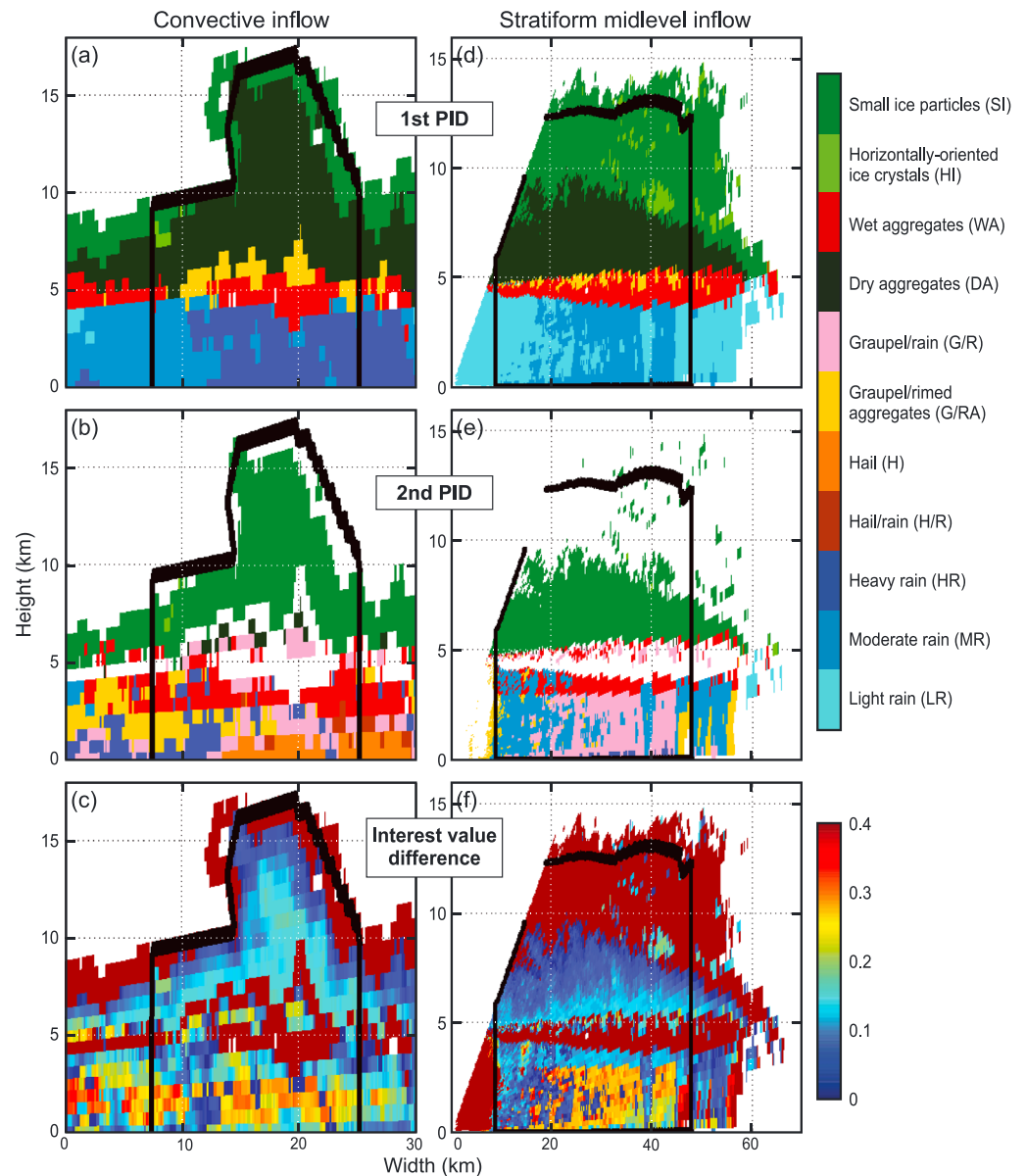
Figure 4. Vertical cross section showing the (a) most likely dominant hydrometeor type (first PID), (b) second most likely dominant hydrometeor type (second PID), and (c) the difference in their interest values for a convective updraft at 0250 UTC on 24 October 2011. The black lines outline the convective updraft region. (d–f) Same as Figures 4a–4c except for a stratiform midlevel inflow region at 0150 UTC on 18 November 2011 and the black lines outline the stratiform region.
