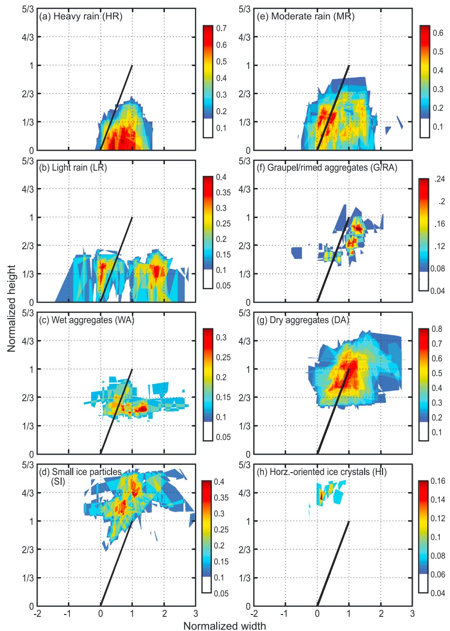
Figure 7. Composites showing the location of (a) heavy rain, (b) light rain, (c) wet aggregates, (d) small ice crystals, (e) moderate rain, (f) graupel/rimed aggregates, (g) dry aggregates, and (h) horizontally oriented ice in convective updrafts. The horizontal and vertical axes are expressed as fractions of the width and height of the convective updraft core and are referred to as the normalized width and height, respectively. The black line represents the composite convective updraft. Shading represents the frequency of each hydrometeor type at that location relative to the convective updraft. The color bar in each panel varies.
