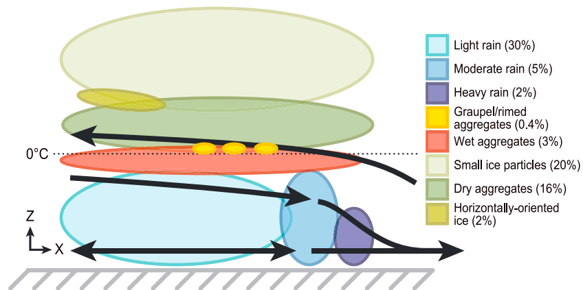
Figure 11. Schematic showing the location of hydrometeor types relative to the stratiform midlevel inflow. The solid black lines in the background represent the stratiform midlevel inflow. The dashed black line indicates the melting level. The gray line represents the surface. The colored regions depict where each hydrometeor is most likely located relative to the stratiform midlevel inflow. The percentages listed in the color bar indicate the average areal coverage of each hydrometeor within RHIs taken through stratiform midlevel inflow.
