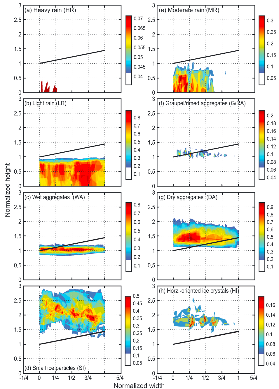
Figure 10. Same as Figure 8 except for stratiform midlevel inflow RHIs that are not associated with a leading convective line. The black line represents the composite stratiform midlevel inflow.
