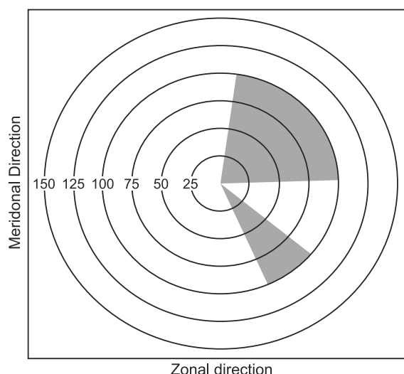
Figure 1. Azimuthal portion of S-PolKa domain containing high-resolution RHI scans within 100 km of the radar shown in gray.
