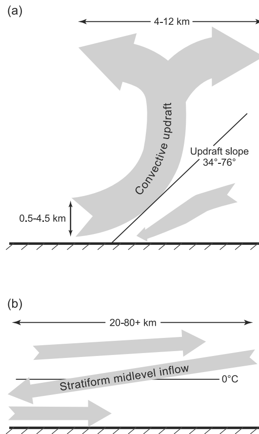
Figure 2. Schematic of airflow through the (a) convective and (b) stratiform portions of MCS over the west Pacific Ocean as observed by airborne Doppler radars during TOGA COARE. The numbers indicate the horizontal velocity of the airflow and the horizontal and vertical extent of the airflow features. The slope of the convective updraft is also indicated in Figure 2a. Figure is based on Kingsmill and Houze [1999] .
