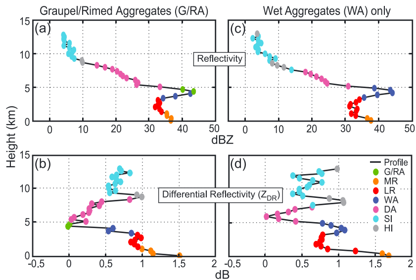
Figure 9. Vertical profile of reflectivity through a portion of the RHI scan in a stratiform midlevel inflow region at 0150 UTC on 18 November 2011 shown in Figure 6 that (a) contains and (c) does not contain graupel/rimed aggregates above the wet aggregate layer. The black line shows the vertical profile of reflectivity. The colored dots represent the location of each hydrometeor type. (b and d) Same as Figures 9a and 9c except that vertical profiles of Z_{DR} are shown.
