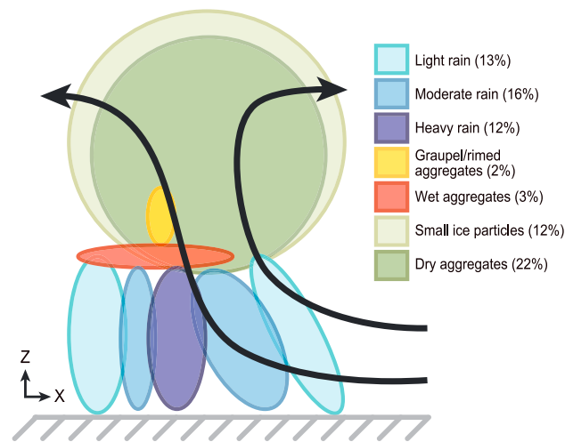
Figure 8. Schematic showing the location of hydrometeor types relative to the convective updraft. The black lines represent the convective updraft. The gray line represents the surface. The colored regions depict where each hydrometeor is most likely located relative to the convective updraft. The percentages listed in the color bar indicate the average areal coverage of each hydrometeor within convective updraft RHIs.
