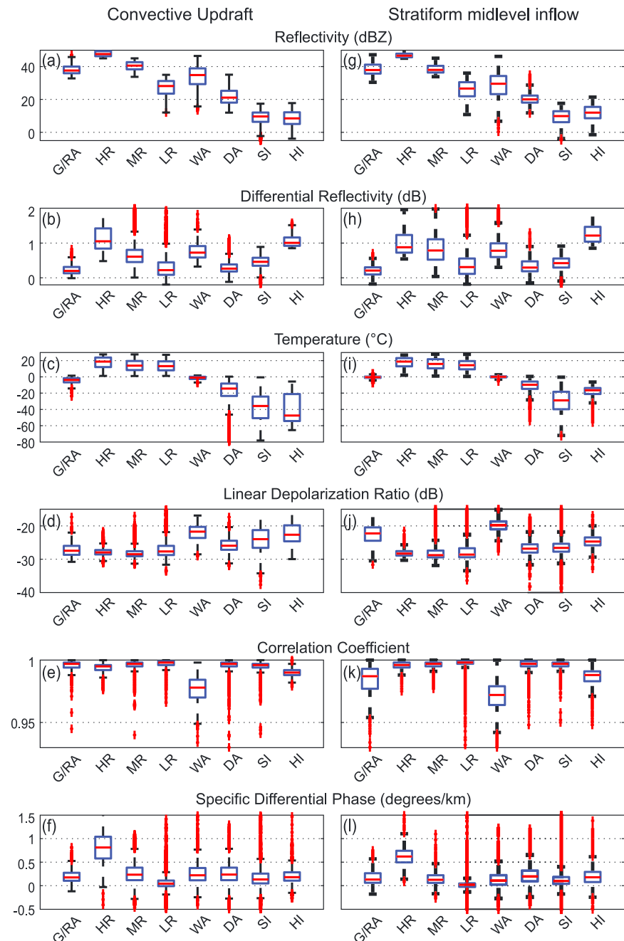
Figure 3. Bar charts showing the distribution of (a) reflectivity, (b) differential reflectivity, (c) temperature, (d) linear depolarization ratio, (e) correlation coefficient, and (f) specific differential phase of all radar volumes in convective updraft regions and contain a contiguous region of graupel/rimed aggregates, heavy rain, moderate rain, light right, wet aggregates, dry aggregates, small ice particles, and horizontally oriented ice crystals. The red line is the median, the blue lines are the 25% and 75% quartiles, the black lines represent 99.3% of the data, and the red stars are outliers. (g–l) Same as Figures 3a–3f except for stratiform midlevel inflow regions.
