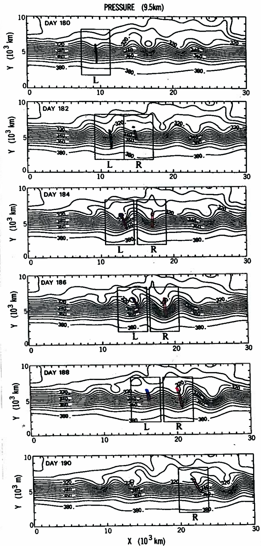
FIG. 7. Evolution of pressure at 9.5 km for days 180 to 190, shown every two days. Contour interval is 5 mb. The boxes in the figure are the areas for which the volume budget shown in Fig. 8 is
