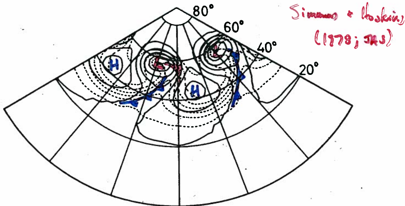
FIG. 1. North polar stereographic plot showing surface pressure (solid contours) and low-level temperature ( \sigma=0.985 , broken contours) after seven days of integration for the wavenumber 6 perturbation to the 45^\circ jet. Contours are drawn at intervals of 2 mb and 4^\circ\text{C} using linear interpolation between values on the computational grid comprising 32 "Gaussian" latitudes and 32 regularly spaced points per 60^\circ longitude. Background lines of latitude and longitude are drawn at intervals of 20^\circ .
