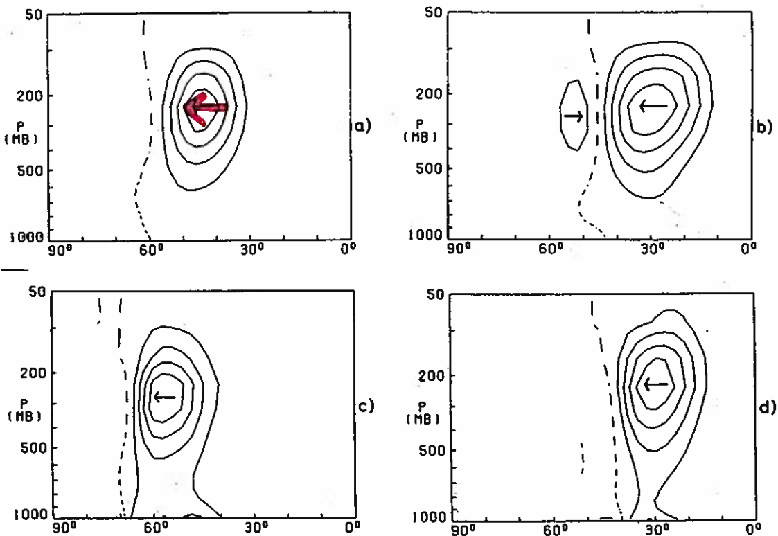
FIG. 8. Meridional cross sections of horizontal eddy momentum fluxes \overline{u'v'} for the same cases as in Fig. 7.
