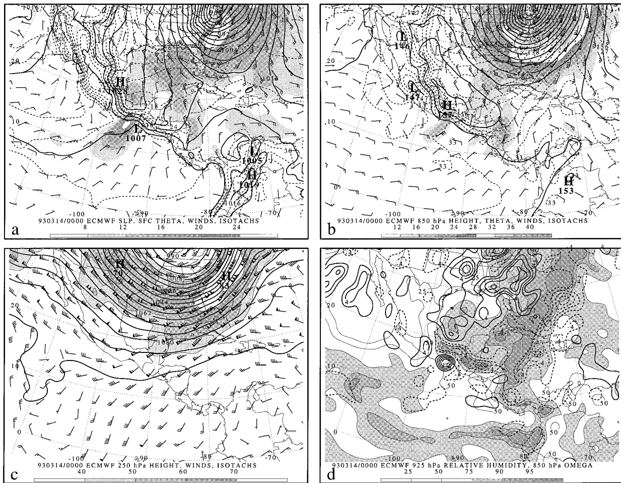
FIG. 5. ECMWF analyses at 0000 UTC 14 March 1993. (a) Sea level pressure (solid lines every 4 hPa), surface potential temperature (dashed lines every 3^{\circ}\text{C} ), 10-m wind (one pennant, full barb, and half-barb denote 25, 5, and 2.5\text{ m s}^{-1} , respectively), and wind speed ( \text{m s}^{-1} , shaded). (b) The 850-hPa geopotential height (solid lines every 3 dam), 850-hPa potential temperature (dashed lines every 3^{\circ}\text{C} ), 850-hPa wind [as in (a)], and wind speed ( \text{m s}^{-1} , shaded). (c) The 250-hPa geopotential height (solid lines every 6 dam), 250-hPa wind [as in (a)], and wind speed ( \text{m s}^{-1} , shaded). (d) The 925-hPa relative humidity (shaded and contoured as noted by scale on bottom of panel) and 850-hPa vertical velocity [every 0.2\text{ Pa s}^{-1} , thick solid lines (thick dashed lines) represent descending (ascending) motion].
