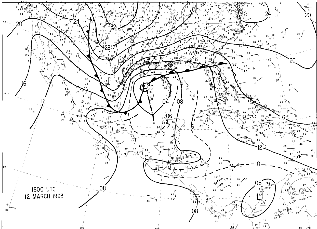
FIG. 13. Manually analyzed surface map for 1800 UTC 12 March. Mean sea level isobars every 4 hPa (solid) and every 2 hPa (dashed, where needed to enhance analysis). Winds: one pennant, full barb, and half-barb denote 25, 5, and 2.5 \text{m s}^{-1} , respectively. Conventional frontal analysis and surface station reports. Dash-dot line represents a surface trough and dash-double-dot line represents location of cloud band 2.
