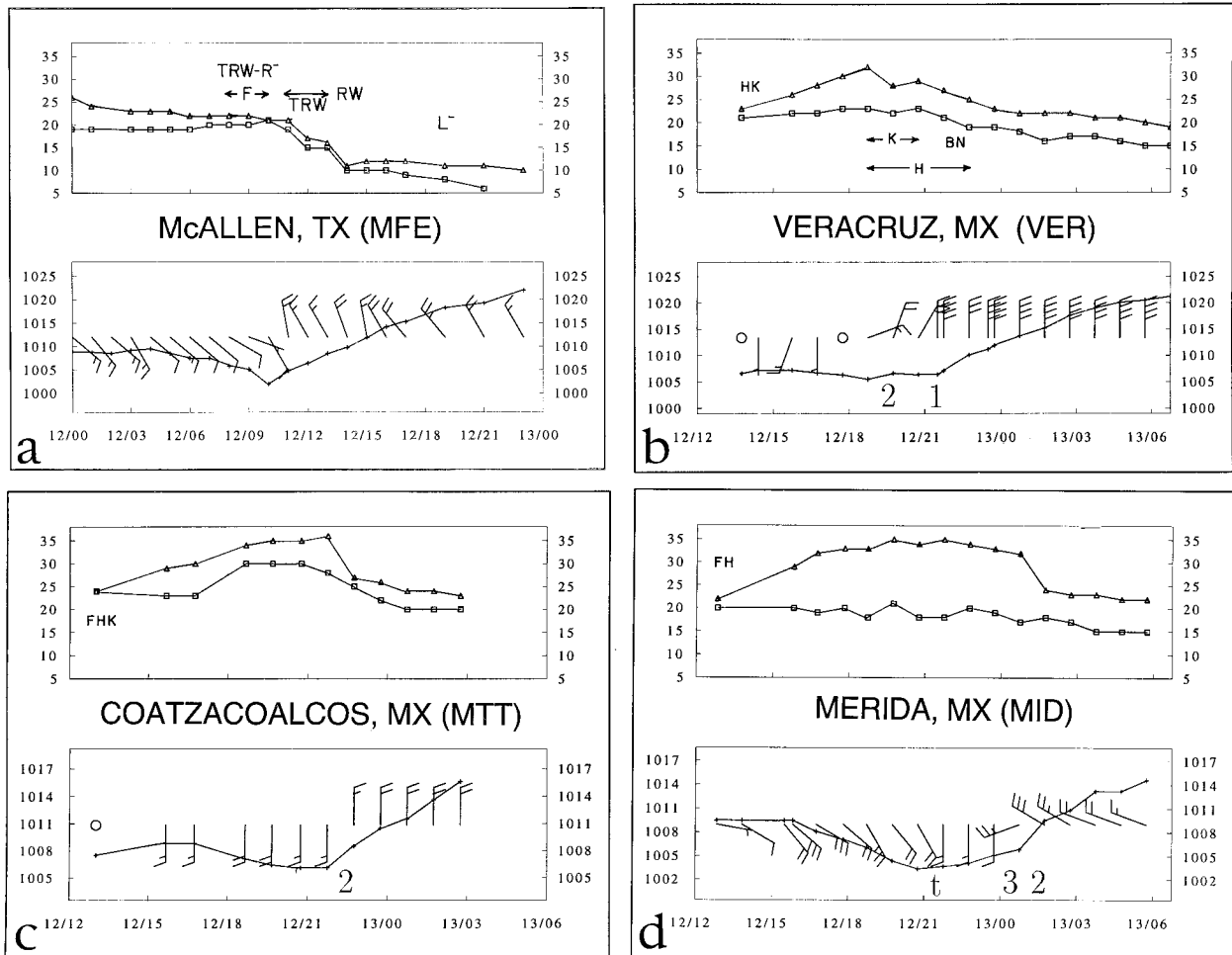
FIG. 11. Meteorograms. Top: temperature (°C, triangles), dewpoint (°C, squares) and significant weather. T = thunderstorms, R = rain, W = showers, A = hail, H = haze, K = smoke, BN = blowing sand, F = fog, L = drizzle, + = heavy, and - = light. Bottom: sea level pressure (hPa) and wind (one pennant, full barb, and half-barb denote 25, 5, and 2.5 \text{m s}^{-1} , respectively). Numbers 1–4 represent passage of cloud bands; t = trough passage. (a) McAllen, Texas (MFE); (b) Veracruz, Mexico (VER, 76691); (c) Coatzacoalcos, Mexico (MTT, 76741); (d) Merida, Mexico (MID, 76644); (e) Puerto Lempira, Honduras (MHPL, 78711); (f) Bahías de Huatulco, Mexico (HUX); (g) Tuxtla Gutierrez, Mexico (TGZ, 76843); and (h) San Jose, Guatemala (MGSJ, 78647).
