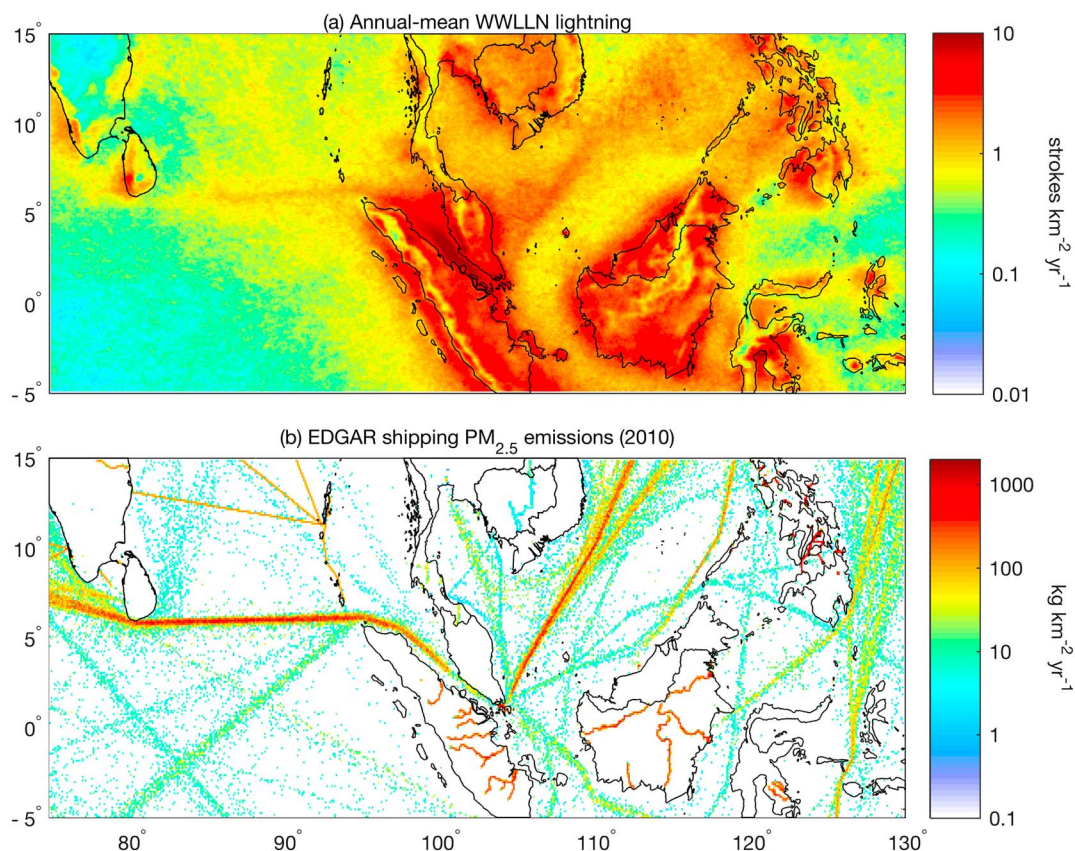
Figure 1. (a) Observed annual-mean WWLLN lightning density for 2005–2016 in the eastern Indian Ocean and the South China Sea. (b) PM_{2.5} shipping emissions estimates from EDGAR database for 2010, both at 0.1^\circ resolution. See text and SI for more details.
