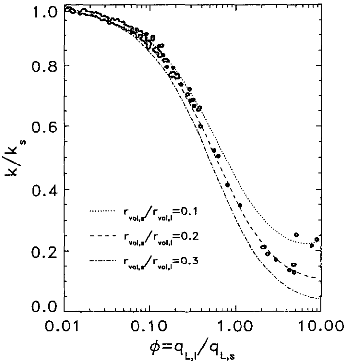
Figure 8. k/k_s against \phi = q_{L,l}/q_{L,s} for the entire dataset (filled circles). Overplotted are the curves using the two-distribution approximation to the size distribution (17) for values of r_{vol,s}/r_{vol,l} = 0.1, 0.2 and 0.3 . In addition, approximations have been made that N_{0,s}/(N_{0,l} + N_{0,s}) = 1 and that the value of k_s inside the square brackets in (17) is a constant equal to 0.7 . Changing this value over the entire range of observed values makes little difference to the final curves obtained. See text for explanation of symbols.
