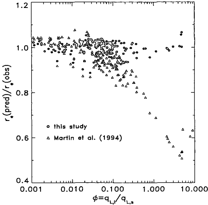
Figure 11. Ratio of predicted to observed effective radius for entire spectrum against ratio of liquid water in large droplets to that in small droplets. The prediction using the parametrization of Martin et al. (1994) (triangles) begins to underestimate the effective radius as q_{L,l}/q_{L,s} rises above 0.05. The underprediction is as great as 50% in the highest drizzle cases. The prediction using the parametrization of (17) (filled circles) predicts the effective radius very well even at high drizzle-water contents. See text for explanation of symbols.
