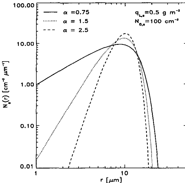
Figure 1. Effect of \alpha upon form of modified gamma function representation of the small-droplet size distribution (see (5)). All three spectra have q_{L,s} = 0.5 \text{ g m}^{-3} and N_{0,s} = 100 \text{ cm}^{-3} and thus r_{\text{vol},s} = 10.61 \text{ } \mu\text{m} (see text).
