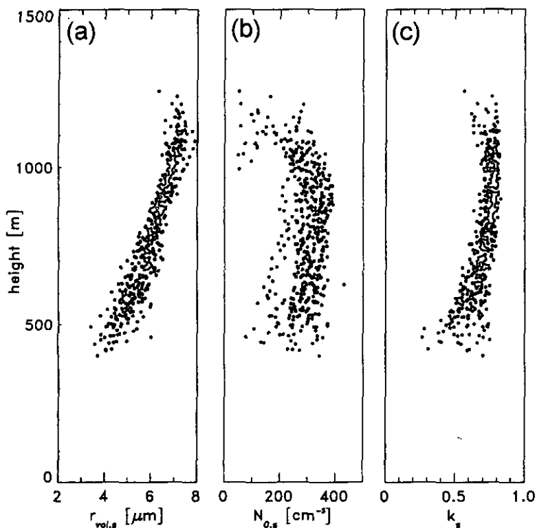
Figure 5. (a) r_{vol,s} , (b) N_{0,s} and (c) k_s (see text) against height for a cloud deck observed over the North Sea on 3 December 1998. Notice how the value of k_s increases with height along with r_{vol,s} , whereas the droplet concentration remains fairly constant with height.
