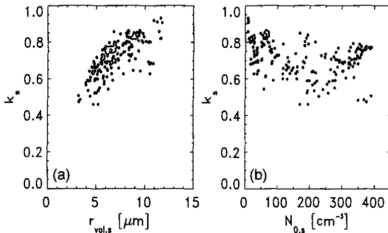
Figure 4. (a) k_s against r_{vol,s} , and (b) k_s against N_{0,s} , for all in-cloud data, showing that the volume radius of the small drops is a better predictor of the value of k_s . See text for explanation of symbols.
