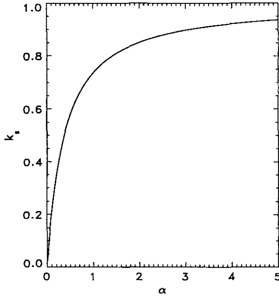
Figure 2. Relationship between k_s and \alpha for the modified Gamma distribution (see text).
