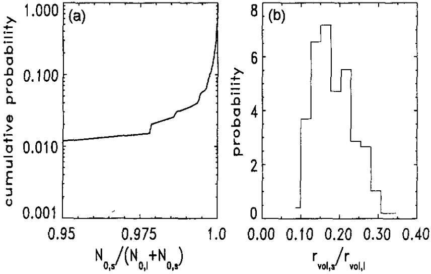
Figure 7. (a) Cumulative distribution of the ratio N_{0,s}/(N_{0,l} + N_{0,s}) . More than 96% of values are larger than 0.99. (b) Distribution of the ratio r_{vol,s}/r_{vol,l} from the entire dataset, where 94% of values are between 0.1 and 0.3. See text for explanation of symbols.
