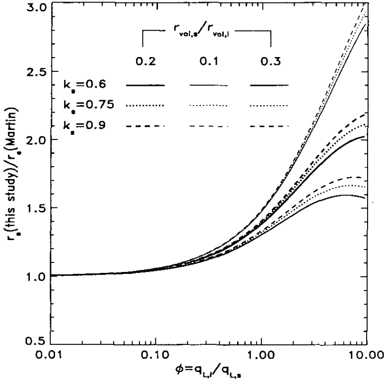
Figure 10. Ratio of the effective radius parametrized using the method presented in this study to that of Martin et al. (1994), as a function of \phi , the ratio of the liquid-water content in the large drops to that in the small drops. The different curves represent different values of k_s and r_{vol,s}/r_{vol,l} , designed to show the sensitivity of the parametrization to changes in these parameters. The parametrization suggested in this study ( r_{vol,s}/r_{vol,l} = 0.2 ) is denoted by the thickest lines. See text for explanation of symbols.
