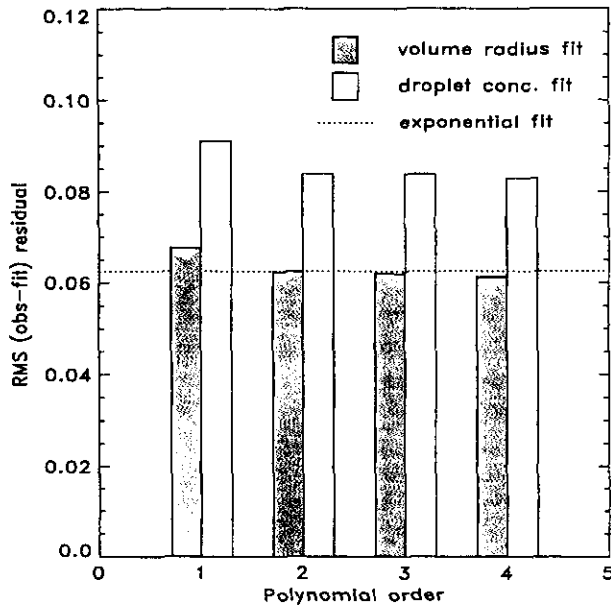
Figure 6. Root-mean-square (r.m.s.) difference between the observed and fitted k_s for polynomial orders 1–4. The solid bar corresponds to the prediction of k_s using r_{\text{vol},s} and the open bar is for that using N_0 . The dotted line is the r.m.s. difference between the observed k_s and that fitted using the exponential form in (18). See text for explanation of symbols.
