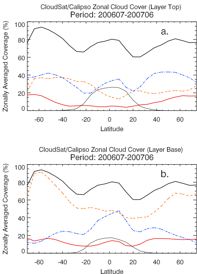
Figure 6. Zonally averaged hydrometeor coverage averaged in 2° latitude bins. (a) Type is defined by layer top altitude. (b) Type is defined by layer base altitude. The averaging period is from July 2006 through June 2007. The thick solid curve includes all hydrometeor layers. The blue dashed curves show coverage of layers with tops (bases) below 3 km mean sea level. The thin solid red curves shows layers with tops (bases) between 3 and 6 km, the dash-dotted blue curves show layers with tops (bases) between 6 and 14 km, and the thin solid black curves show layers with tops (bases) above 14 km. Multiple layers are counted in Figure 6b, but only the highest top is counted in Figure 6a. In Figure 6a the thin black curve counts only layers with tops above 14 km and that have thickness less than 3 km.
