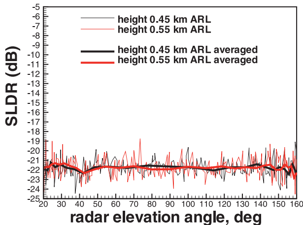
FIG. 2. Instantaneous and averaged measurements of SLDR at 0.45 and 0.55 km ARL during the RHI scan toward the SPL ( az = 87.1^\circ ) when observing freezing drizzle at 1800 UTC 16 Jan 2011.
