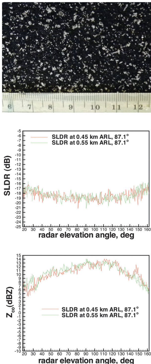
FIG. 12. (top) A particle photograph (small ruler ticks are millimeters) and (middle) SLDR, and (bottom) Z_{co} elevation angle dependences for RHI scans at 1750 UTC 31 Jan 2011 when some columnar particles were present in the hydrometeor mixture.
