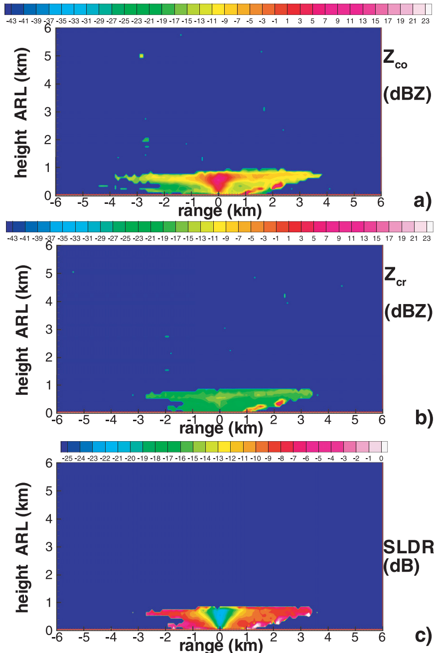
FIG. 5. SWACR measurements of (a) copolar and (b) cross-polar reflectivity and (c) SLDR during the RHI scan toward the SPL ( az = 87.1^\circ ) when observing pristine dendrites at 1700 UTC 11 Feb 2011.
