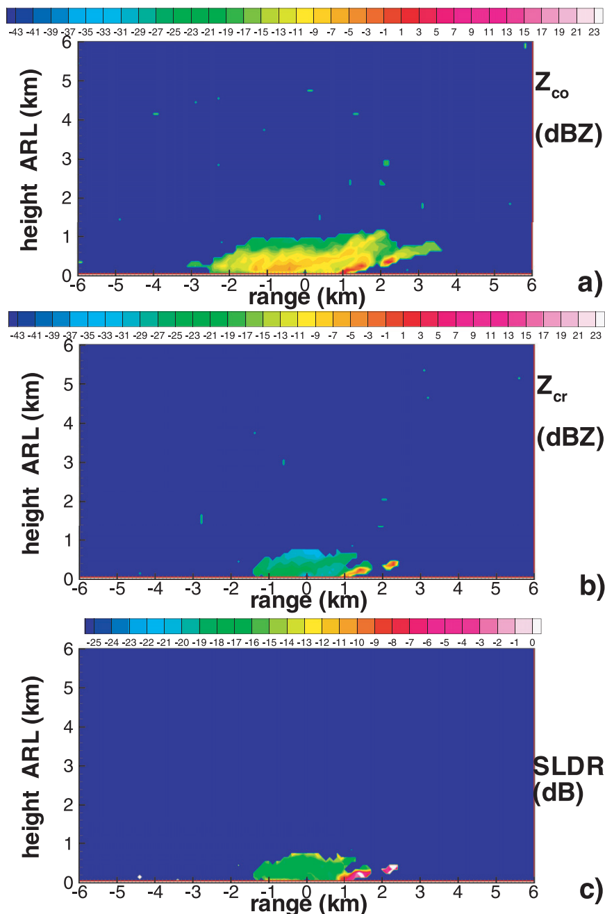
FIG. 14. SWACR measurements of (a) copolar and (b) cross-polar reflectivity and (c) SLDR during the RHI scan toward the SPL ( az = 87.1^\circ ) when observing predominantly columnar crystals at 0341 UTC 4 Mar 2011.
