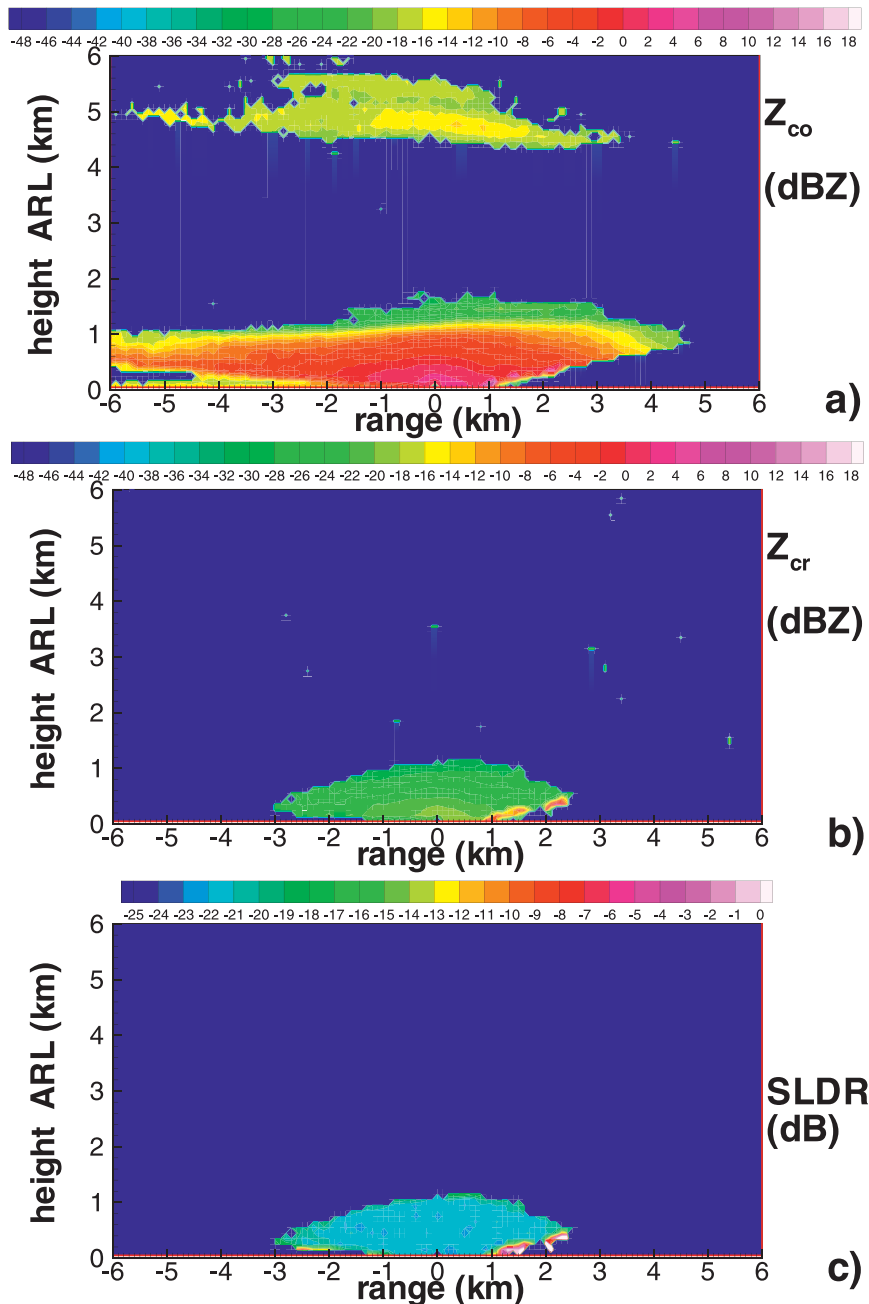
FIG. 1. SWACR measurements of (a) copolar and (b) cross-polar reflectivity and (c) SLDR during the RHI scan toward the SPL ( \text{az} = 87.1^\circ ) when observing freezing drizzle at 1800 UTC 16 Jan 2011.
