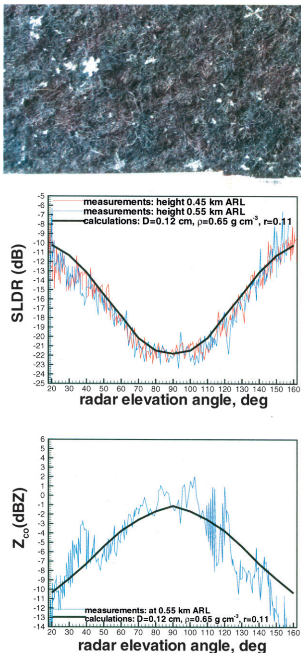
FIG. 8. (top) A particle photograph (small ruler ticks are millimeters), (middle) SLDR, and (bottom) Z_{co} data during the RHI scan shown in Fig. 7.
