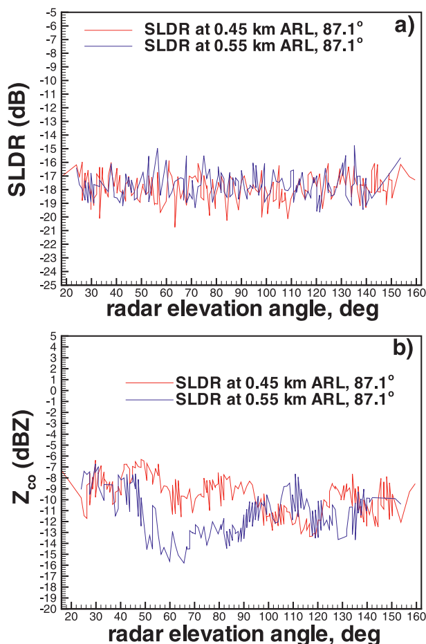
FIG. 15. (a) SLDR and (b) Z_{co} elevation angle dependences for the RHI scan toward the SPL at 0341 UTC 4 Mar 2011 when columnar particles were the predominant habit.
