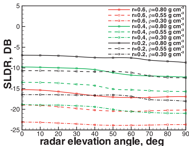
FIG. 13. Model calculations of SLDR vs radar elevation angle for columnar (prolate)-type particles for different aspect ratio and density assumptions, D = 1 mm.
