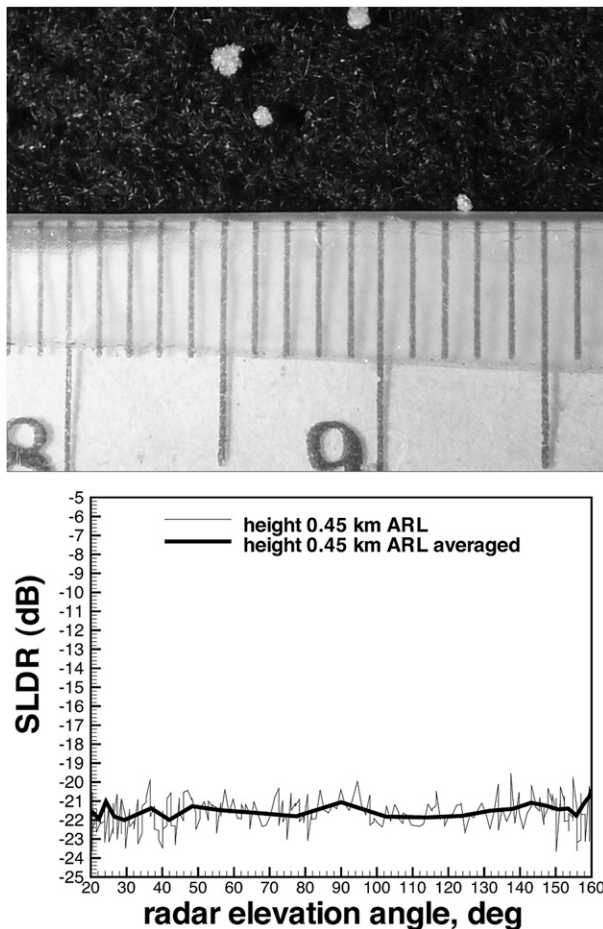
FIG. 4. (top) A particle photograph (small ruler ticks are millimeters) and (bottom) the instantaneous and averaged measurements of SLDR at 0.45 km ARL during the RHI scan toward the SPL ( az = 87.1^\circ ) when observing round graupel (for corresponding RHI scans see Fig. 3).
