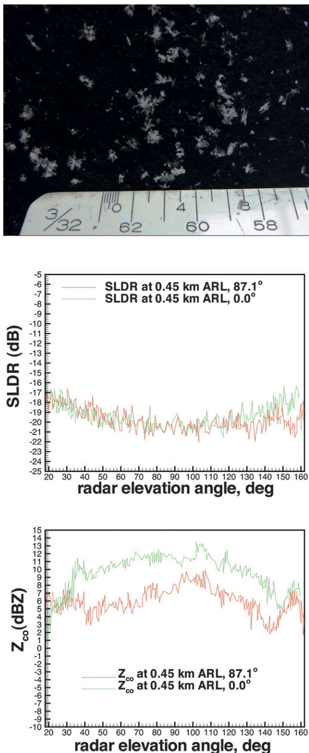
FIG. 11. (top) A particle photograph (the big ticks on the ruler are 0.47 cm apart), (middle) SLDR, and (bottom) Z_{co} elevation angle dependences for RHI scans at 2130 UTC 31 Jan 2011 when aggregates of dendrites were the predominant particle type.
