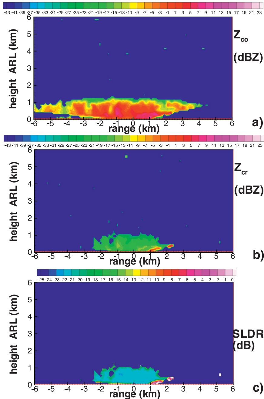
FIG. 3. SWACR measurements of (a) copolar and (b) cross-polar reflectivity and (c) SLDR during the RHI scan toward the SPL ( az = 87.1^\circ ) when observing round graupel at 2228 UTC 14 Jan 2011.
