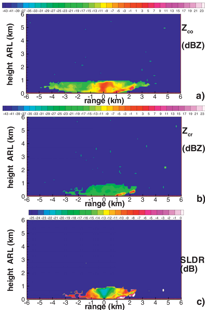
FIG. 7. SWACR measurements of (a) copolar and (b) cross-polar reflectivity and (c) SLDR during the RHI scan toward the SPL ( az = 87.1^\circ ) when observing lightly rimed dendrites at 1823 UTC 26 Jan 2011.
