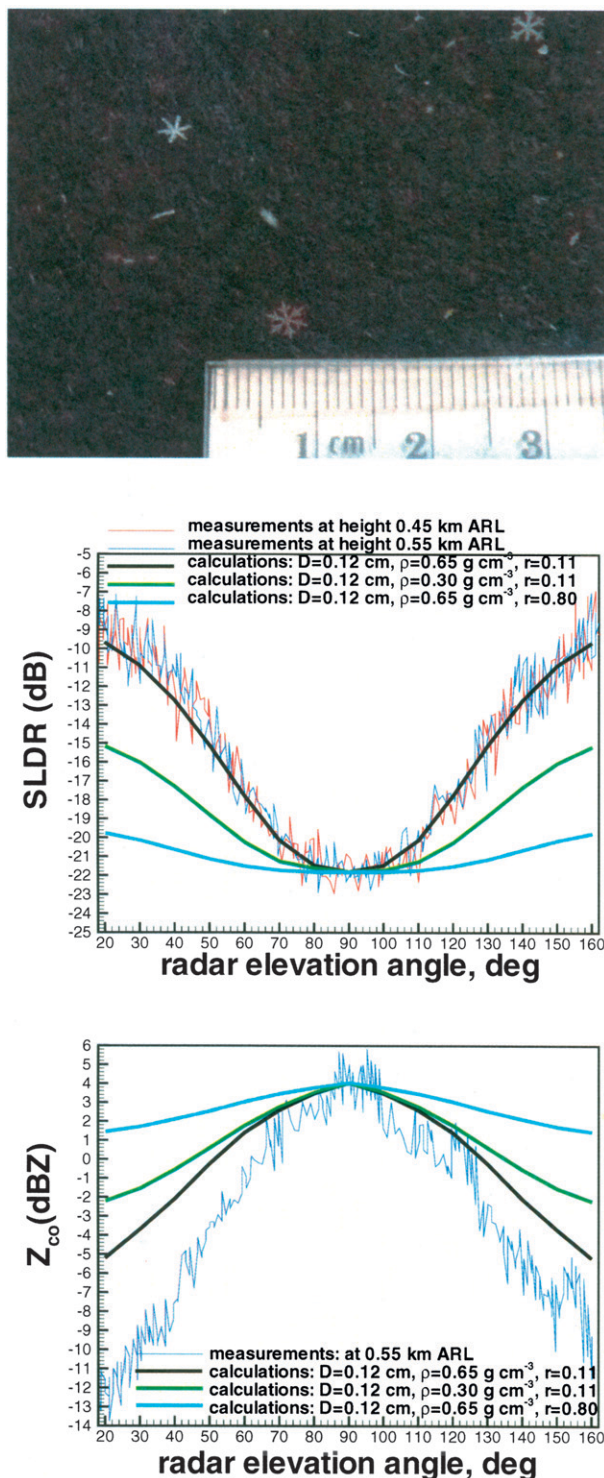
FIG. 6. (top) A particle photograph, (middle) SLDR, and (bottom) Z_{co} measurements and calculations for the RHI scan shown in Fig. 5.
