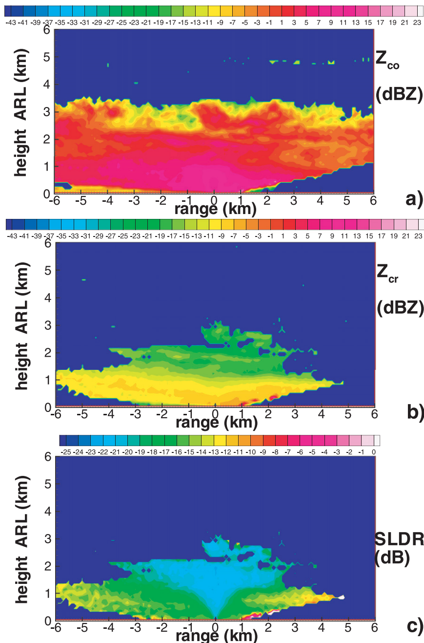
FIG. 9. SWACR measurements of (a) copolar and (b) cross-polar reflectivity and (c) SLDR during the RHI scan toward the SPL ( az = 87.1^\circ ) when observing moderately rimed stellar and dendritic crystals with smaller irregulars and hexagonal plates at 2036 UTC 25 Jan 2011.
