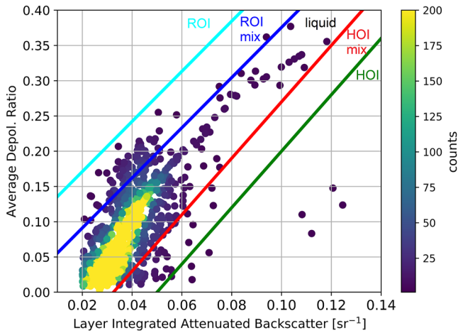
Figure 1. Cloud base layer \gamma versus \delta_L points for cloud top heights <3 km, cloud base height >450 m and cloud top temperature >0°C (i.e., this is for warm/liquid clouds). Lines/categories that identified Horizontally Oriented Ice (HOI), randomly-oriented ice crystals (ROI) and liquid are as defined by Mace et al. (2020); see text. The colorbar shows density of counts/number of 5-min observations. Uncertainty is estimated to be about \pm 2.5\% by considering the percentage of points above/below the liquid boundaries (blue and red lines).
