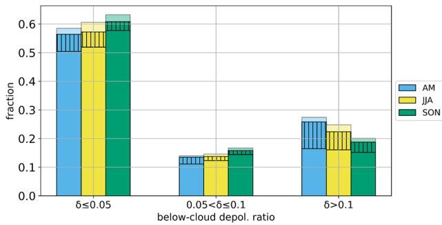
Figure 3. Fraction of below-cloud precipitation for clouds with CTT < 0^\circ C in each season by (i) cloud-base phase (dark color bars = liquid, striped dark color bars = mix/uncertain, light color bars = ice) and (ii) layer-averaged \delta_L (horizontal axis).
