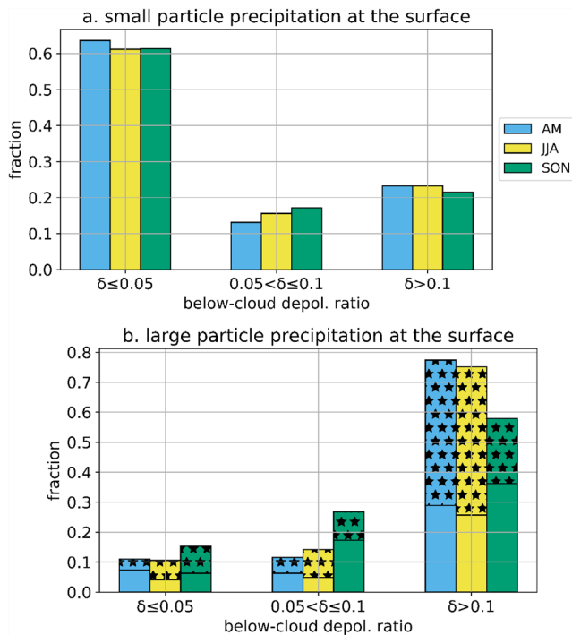
Figure 6. (a) Small-particle precipitation at the surface by season, split into different lidar \delta_L phase regimes in the layer CBH–200 m through CBH–100 m. (b) Same as (a), but for large particles. Precipitation for both warm- and cold-topped clouds is included. Solid colors represent rain, stars represent mixed/frozen as designated by the surface disdrometer. Phase specification is only possible for large particles (diameters > \sim 1 mm) with the Parsivel disdrometer.
