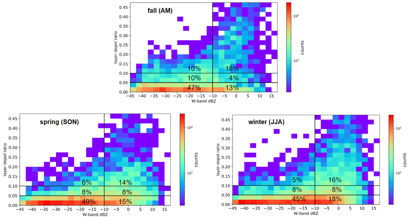
Figure 4. 2D histograms of \delta_L versus dBZ for precipitation below the bases of cold clouds, with the percentage of counts above/below -10 dBZ and in each \delta_L phase regime.
