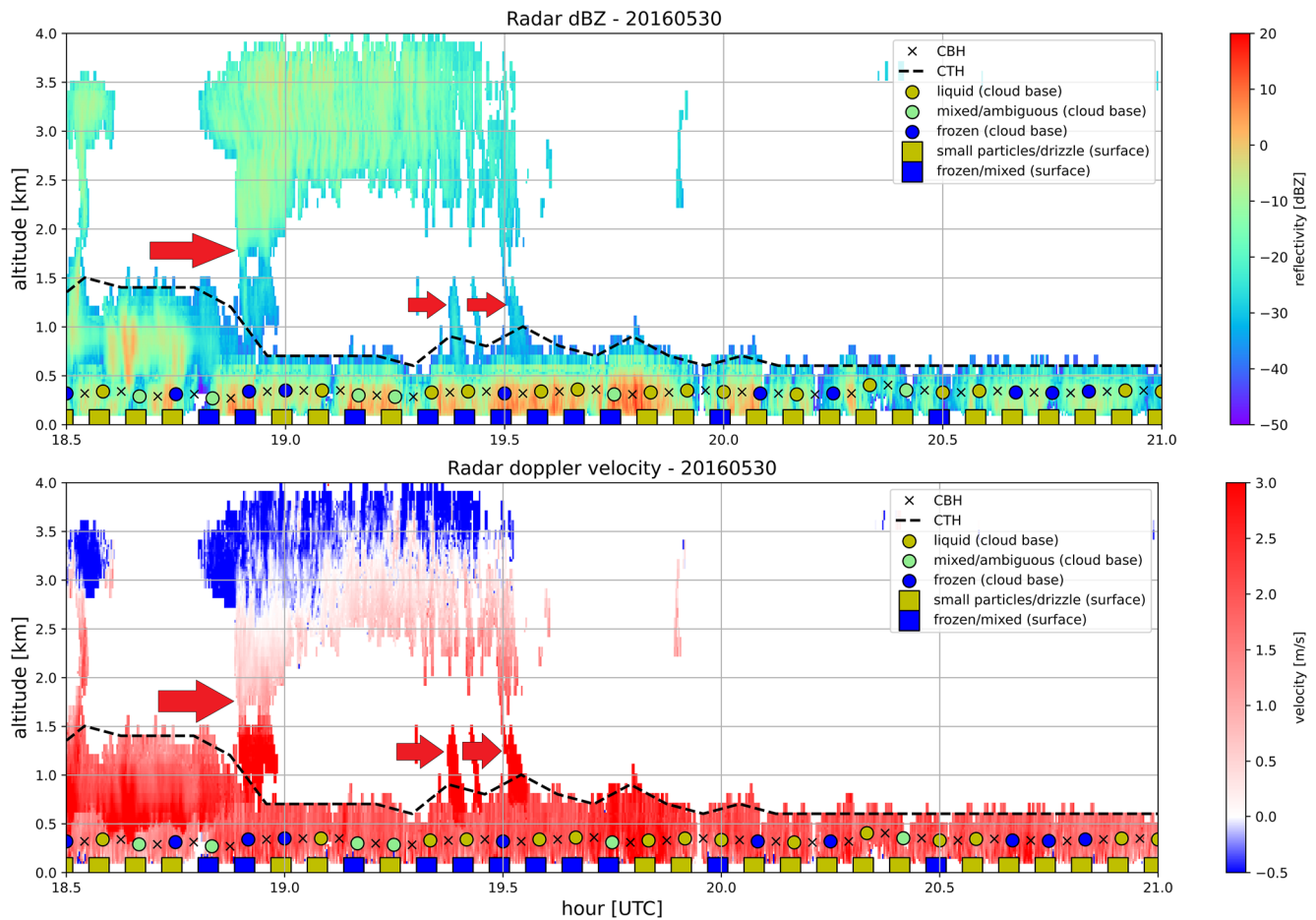
Figure 2. Example of a seeder-feeder event in which a higher cloud forms ice particles that seed precipitation in the lower cloud layer. Arrows overlaid on the plot point to obvious seeder-feeder instances. Cloud base height is marked by x's, cloud top height by dashed lines. The phase of particles at cloud base are given by dots (color-coded by phase). Precipitation phase at the surface (squares) are from the Macquarie Island Cloud and Radiation Experiment radar-disdrometer blended surface data set (Tansey et al., 2022a).
