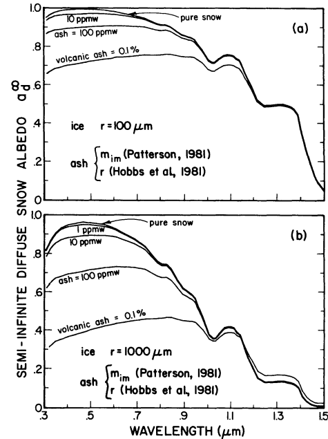
Fig. 7. Effect of Mount St. Helens ash on snow albedo for diffuse incidence: (a) snow grain size r = 100 \mu\text{m} ; (b) r = 1000 \mu\text{m} . Ash parameters are described in the text.
