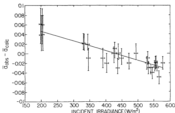
Fig. 13. Effect of cloud cover on spectrally integrated snow albedo. The difference between observed and calculated spectrally integrated albedos is plotted versus incident irradiance (which is here approximately proportional to atmospheric transmissivity, because the measurements were all made between 1100 and 1400) for snow in the Cascade Mountains. 'Calculated' albedos were calculated by Grenfell et al. [1981] using observed spectral albedos with a fixed incident spectral distribution characteristic of an intermediate cloud thickness. The straight line is a least squares fit to the data points. (Figure 5 of Grenfell et al. [1981]. Reprinted by permission of Elsevier.)
