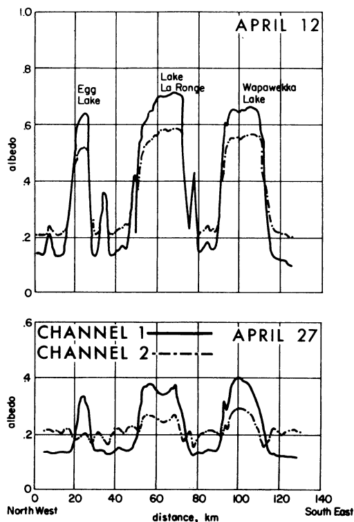
Fig. 20. Traces of reflectance measured from satellite by NOAA scanning radiometer across three lakes in Saskatchewan on two different days in visible channel 1 ( 0.5 – 0.7 \mu\text{m} ) and near-IR channel 2 ( 0.7 – 1.0 \mu\text{m} ). (Figure 10 of Dozier et al. [1981].)
