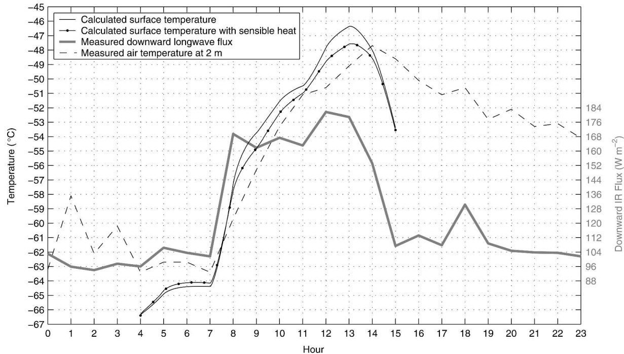
FIG. 19. Results of the snow-temperature model during the warming in Fig. 18 both with and without sensible heat flux. Also shown is the measured T_2 and the downward longwave flux; the latter was used as an input into the model.
