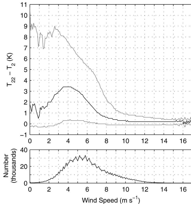
FIG. 10. Median inversion strength (dark line) in the 2- to 22-m layer as a function of wind speed in winter; lighter lines are the 10th and 90th percentiles. The lower panel shows the number of observations in each bin of width 0.1 \text{ m s}^{-1} .
