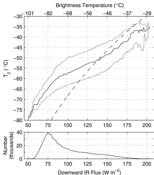
FIG. 6. Median 2-m air temperature (dark line) as a function of downward infrared flux (or corresponding brightness temperature of the sky) in winter; lighter lines are the 10th and 90th percentiles. The dashed curve shows where T_2 would be equal to the brightness temperature of the sky (actual radiative equilibrium between the surface and the sky would occur slightly to the left of this curve because the surface is generally colder than the air at 2 m, and because the surface has an emissivity slightly less than 1). The lower panel shows the number of observations in each bin of width 1 W m^{-2} .
