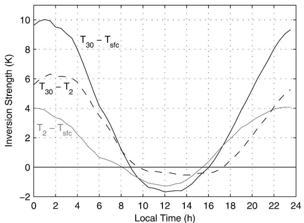
FIG. 21. Half-hourly mean inversion strength across the three available layers at Dome C Station for the 2004/05 summer. Time is given in local standard time, UTC+8
