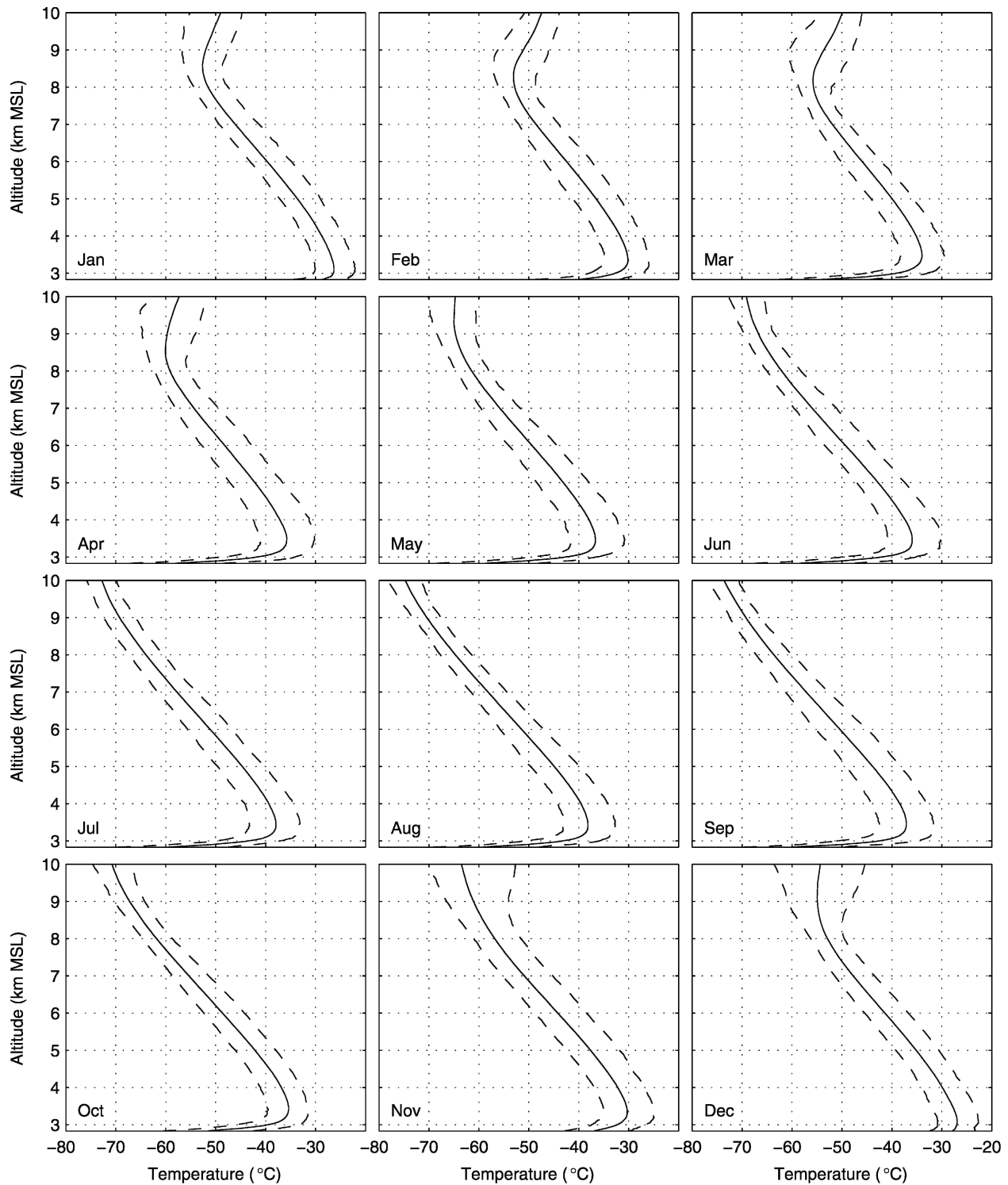
FIG. 16. Same as Fig. 15, but only the lowest 10 km.
