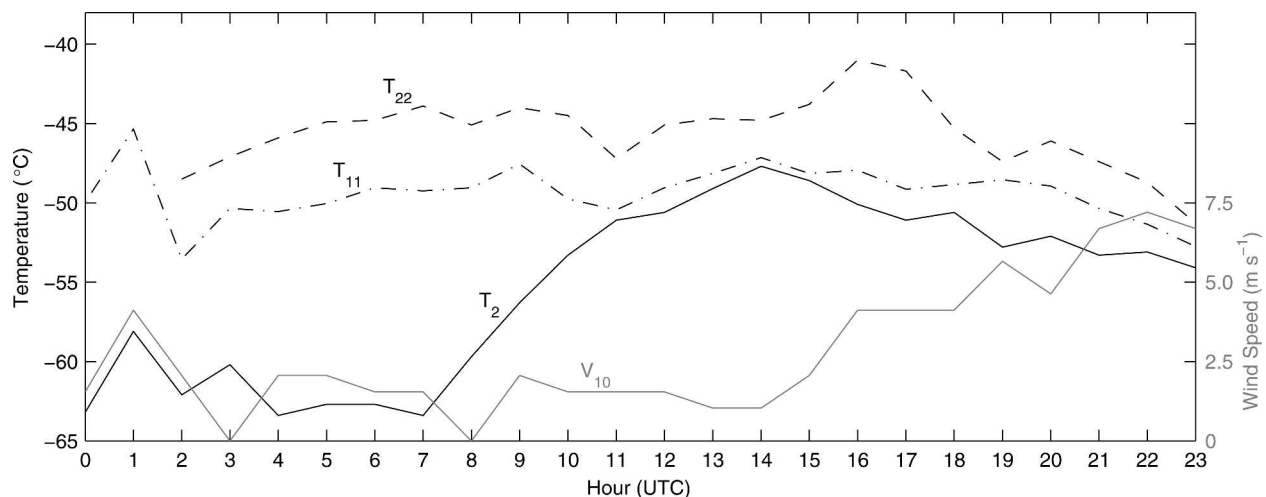
FIG. 18. Air temperatures at 2, 11, and 22 m, and 10-m wind speed ( V_{10} ) at South Pole on 8 Sep 1992.
