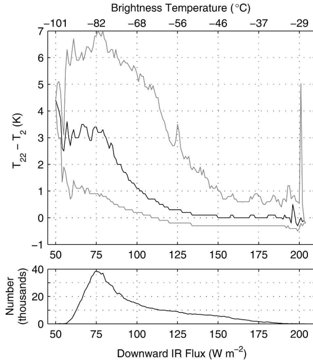
FIG. 8. Median inversion strength (dark line) in the 2- to 22-m layer as a function of downward infrared flux (or corresponding brightness temperature of the sky) in winter; lighter lines are the 10th and 90th percentiles. The lower panel shows the number of observations in each bin of width 1 \text{W m}^{-2} .
