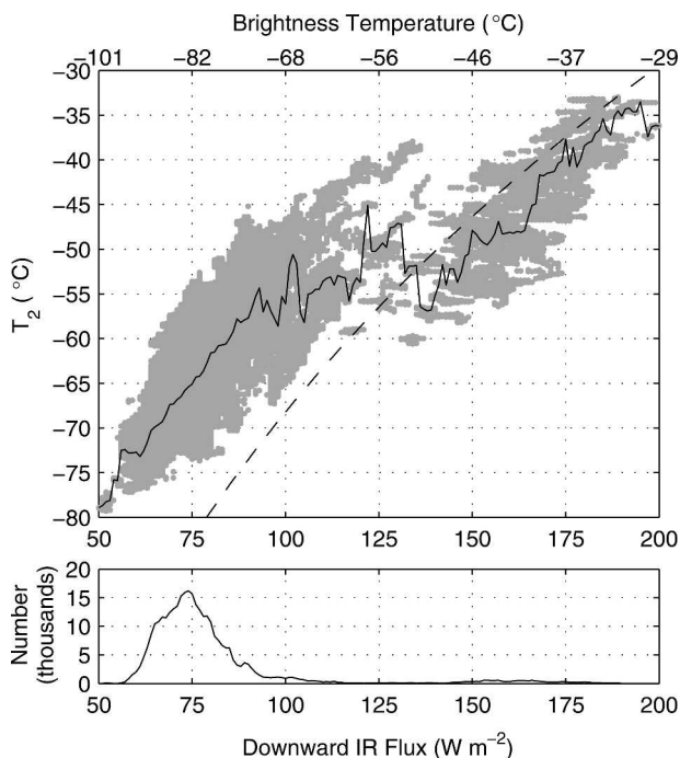
FIG. 7. A scatterplot of filtered, winter T_2 data (gray area) and the median (solid line) of these data as a function of downward infrared flux (or corresponding brightness temperature of the sky). The dashed curve shows where T_2 would be equal to the brightness temperature of the sky. The lower panel shows the number of observations in each bin of width 1 W m^{-2} .
