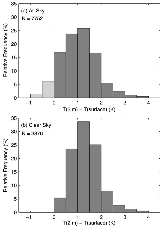
FIG. 14. Relative frequencies of observed temperature differences between 2 m and the surface during the 2001 polar night. (a) The data from all-sky conditions and (b) those from clear-sky conditions.
