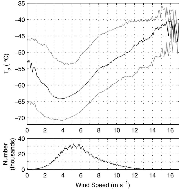
FIG. 9. Median 2-m temperature (dark line) as a function of wind speed in winter; lighter lines are the 10th and 90th percentiles. The lower panel shows the number of observations in each bin of width 0.1 \text{m s}^{-1} .
