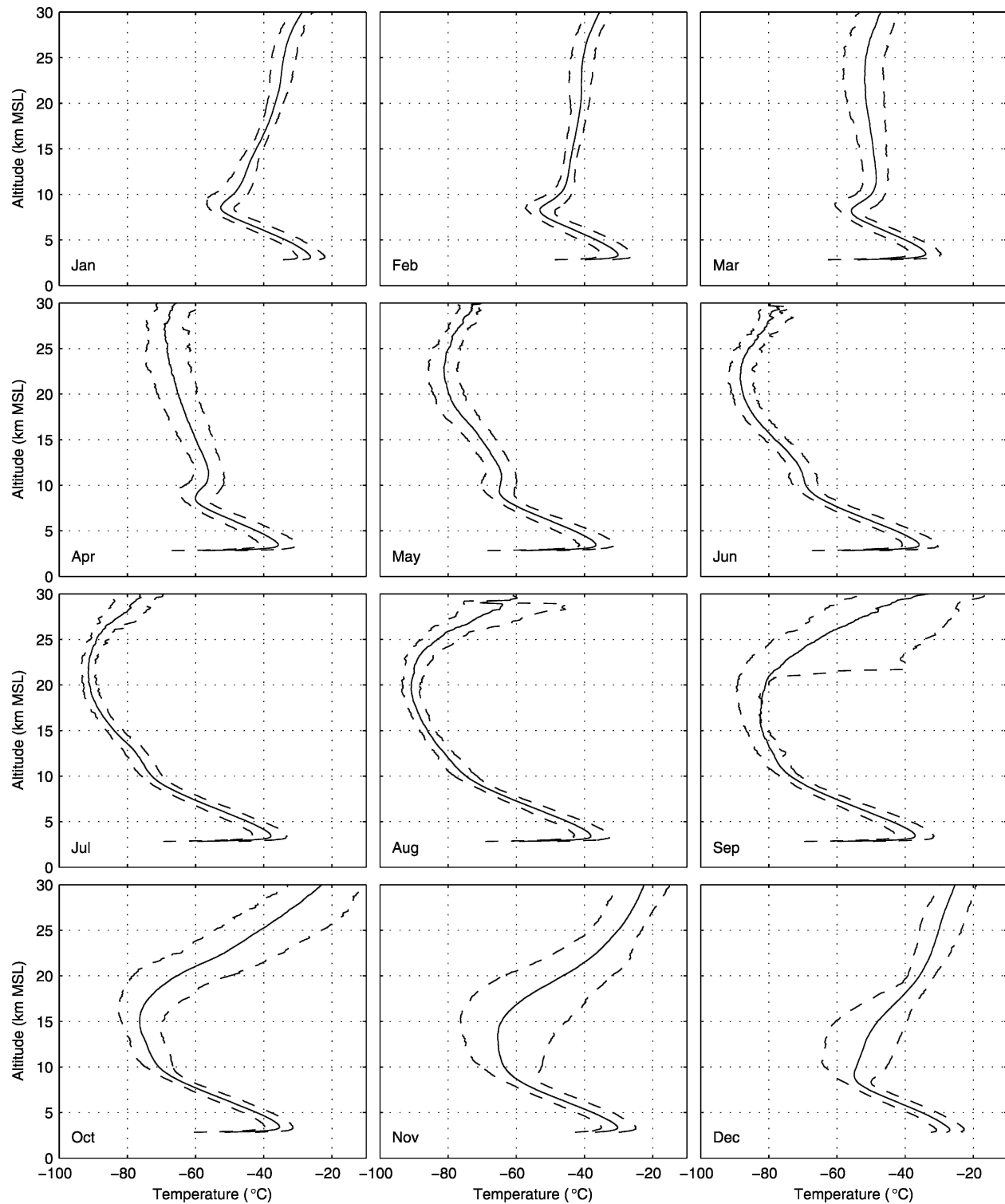
FIG. 15. The monthly mean (solid line) atmospheric temperature profiles from 2 m above the surface to 30 km MSL over South Pole. The dashed lines show the 10th and 90th percentiles of temperature at each height. Radiosonde data begin 55 m above the surface (2890 m), and temperatures from a tower are used at 2 and 22 m. Data from 1994 to 2003 were used.
