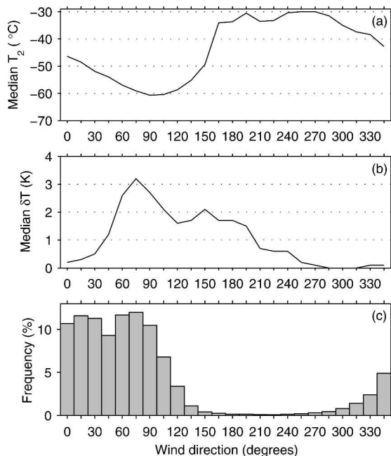
FIG. 12. (a) The median 2-m air temperature and (b) median inversion strength between 2 and 22 m as functions of wind direction. The frequency of winds from each direction is shown in (c). Data are for the entire year and were grouped into 15° bins centered on 000°, 015°, ..., 345°.
