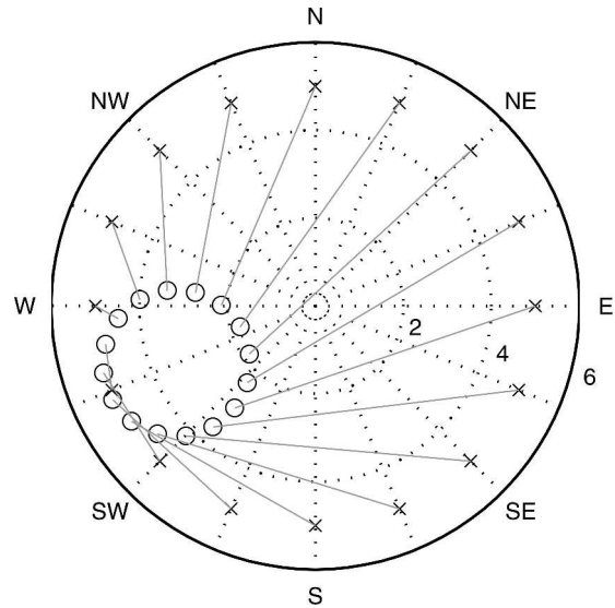
FIG. 11. Winds generated by the inversion under various synoptic conditions. The crosses indicate end points of geostrophic wind vectors at the top of the inversion. Each is connected by a line to a circle that indicates the end point of the resulting 10-m wind calculated with the inversion wind model using the corresponding geostrophic wind to specify the synoptic pressure gradient. For example, with a geostrophic wind at the top of the inversion of 5 \text{ m s}^{-1} from the south (indicated by the cross at the top of the plot), the inversion wind model predicts a 10-m wind of just over 2 \text{ m s}^{-1} from the east (indicated by the circle that is attached to the cross at the top). Radial grids are at 2 and 4 \text{ m s}^{-1} . The downslope direction is 285^\circ .
