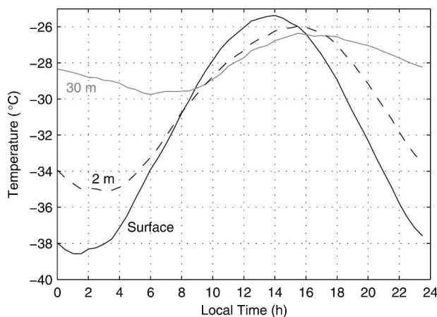
FIG. 20. Half-hourly mean surface temperature and air temperature at 2 and 30 m at Dome C Station for the 2004/05 summer. Time is given in local standard time, UTC+8
