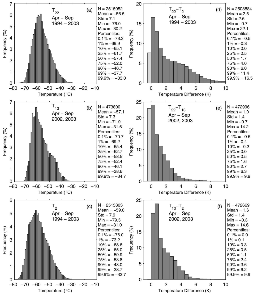
FIG. 5. As in Fig. 4, but for winter months. Note that the abscissas are on fixed scales for comparison (the same scales used in Fig. 4), but the ordinates vary between plots to maximize readability.
