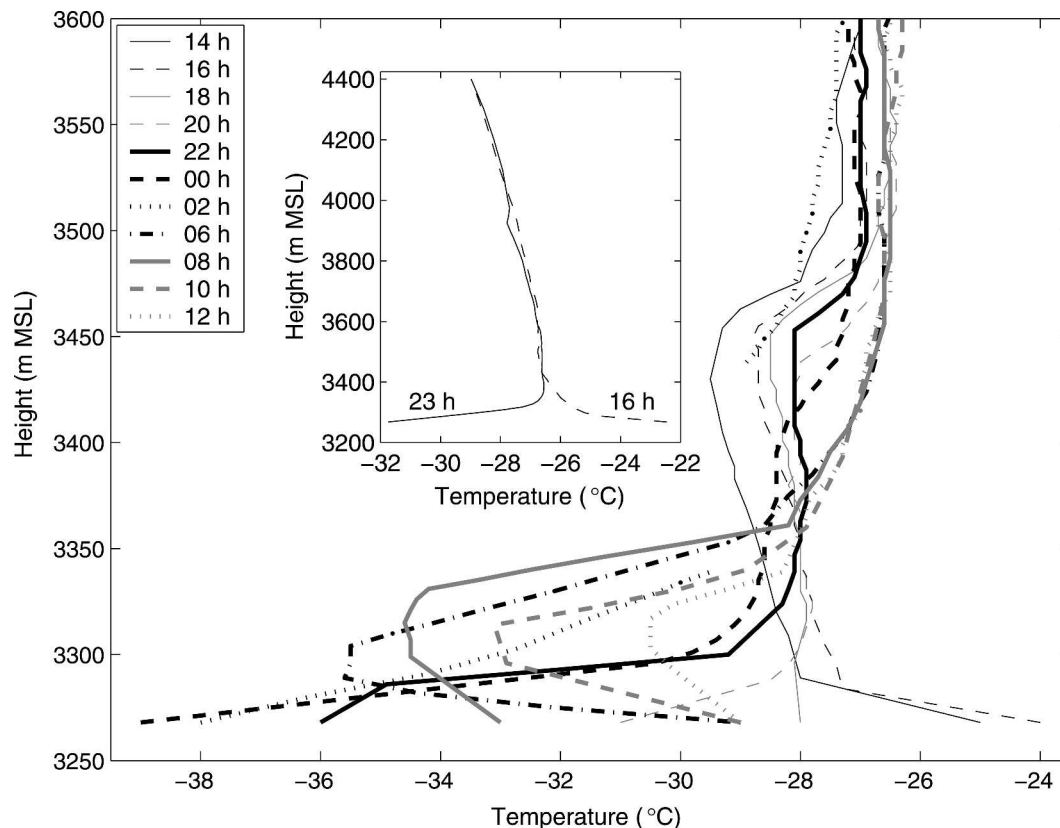
FIG. 22. The main panel shows soundings from Dome C taken every 2 h from 1400 LST 24 Jan 2004 to 1200 LST 25 Jan 2004. The surface is at 3266 m, and the lowest point is the 2-m air temperature measured at the time of launch. The 0400 LST sounding is not available, and the 0200 LST sounding is missing data from approximately 3350 to 3450 m. The inset panel shows the mean temperature profile from all soundings at Dome C taken in the hour centered on 1600 LST (dashed line) and on 2300 LST (solid line). Twenty soundings taken between mid-Dec 2003 and the end of Jan 2004 went into each of these two mean profiles. All times are given in local standard time, UTC+8.
