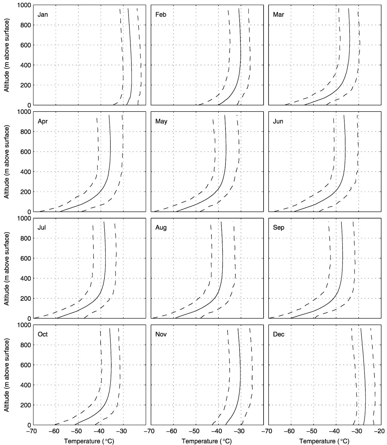
FIG. 17. Same as Fig. 15, but only the lowest 1 km above the surface.
