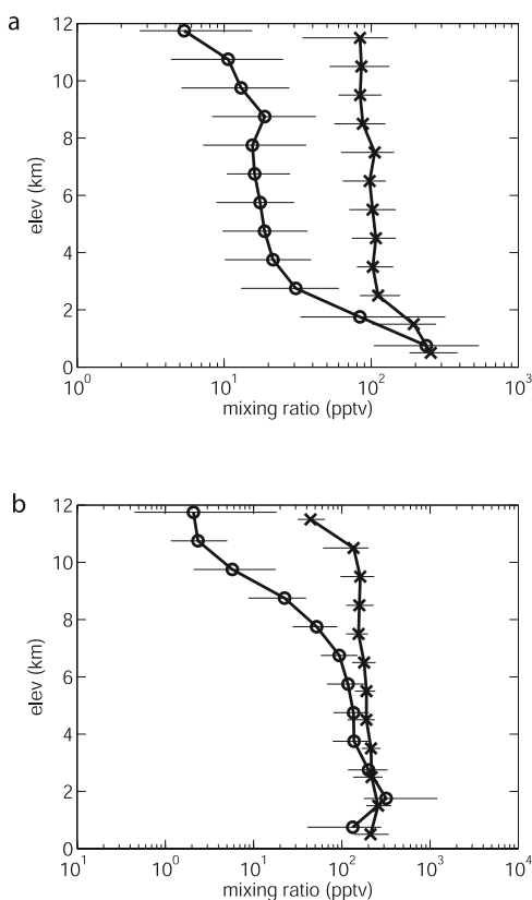
Figure 2. Modeled (circle) vs. measured (x) profiles for (a) acetaldehyde and (b) peroxyacetic acid. Marks are bin medians, lines are interquartile range. Model predictions, offset by 0.25 km for clarity, are based on the photochemical box model of Crawford et al. [1999], and assume a PAA lifetime of \sim 20 days (upper limit).
